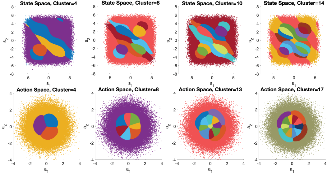
Figure 5: Row 1: Learned state abstractions with varying clustering sizes by top- r method; Row 2: Learned action abstractions with varying clustering sizes by top- r method.
