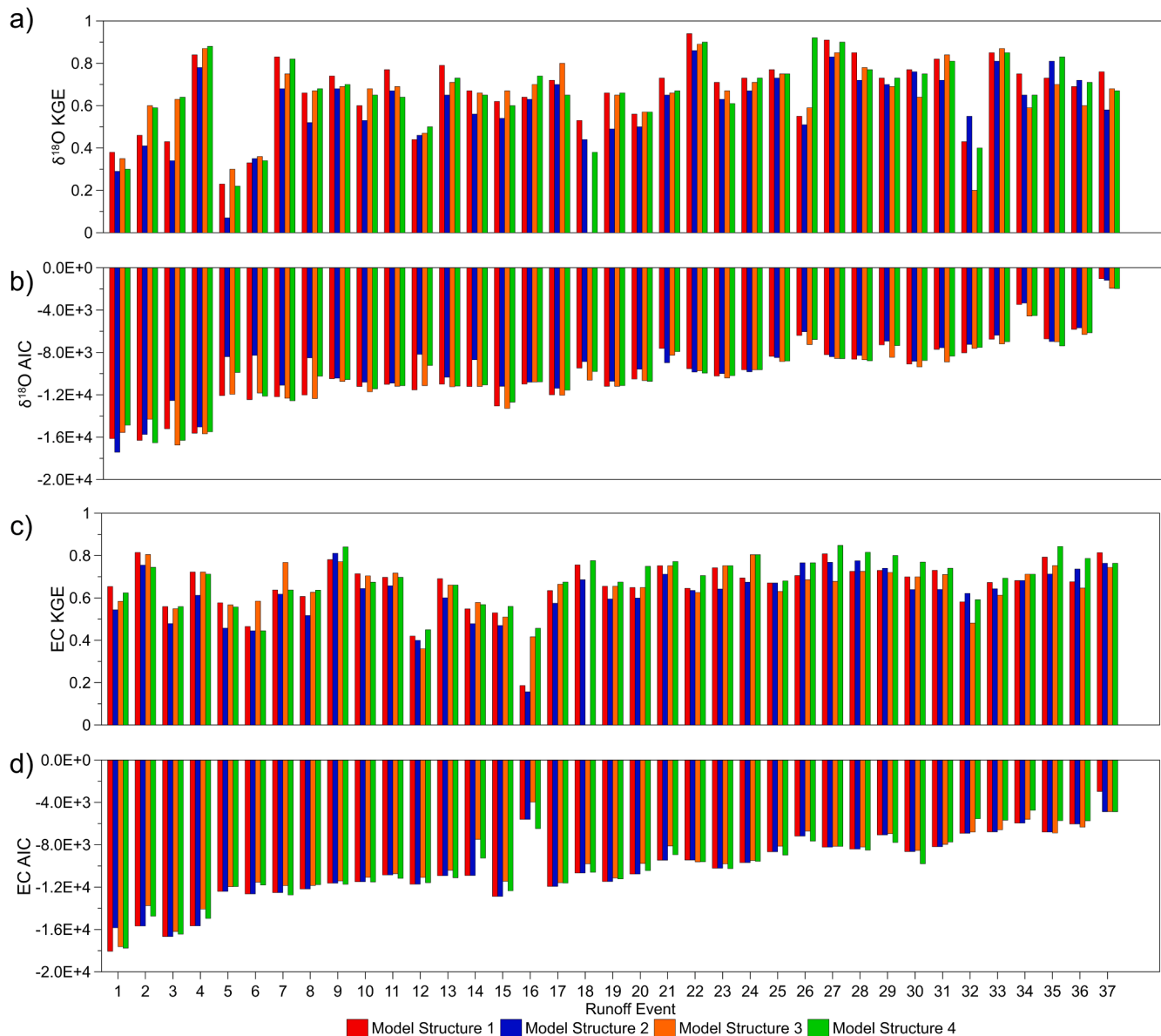
Fig. 3. Best model performance metrics (KGE and AIC) of flow partitioning using high resolution \delta^{18}\text{O} and EC data with each model structure. Red, blue, orange, and green bars correspond to model structures 1, 2, 3, and 4, respectively. Subplots a) and b) correspond to \delta^{18}\text{O} calibration, and (c) and (d) correspond to EC calibration. (For interpretation of the references to colour in this figure legend, the reader is referred to the web version of this article.)
