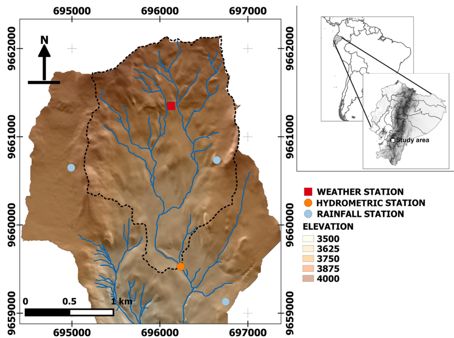
Fig. 1. Map of the study site located at the Zhurucay Ecohydrological Observatory (ZEO) in south Ecuador showing the hydrometeorological monitoring setup.
