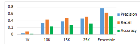
Figure 2: Discord Lengths and Ensemble Model evaluation
