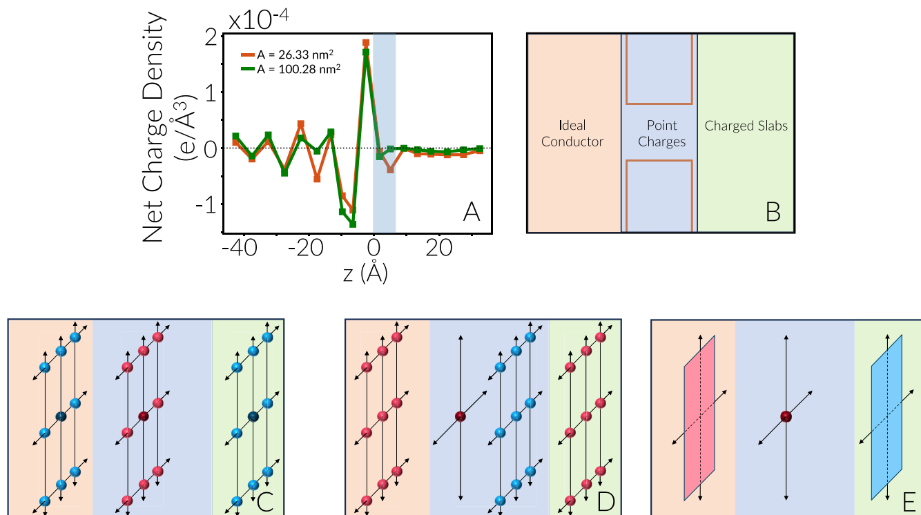
FIG. 8. (a) Net charge density as a function of distance from the pore mouth in the F_{0,1} basin. (b) Schematic representation of the separation system, comprised of the conducting feed, the membrane (which can include extra point charges) and the dielectric filtrate (that contains the leading chloride). (c) and (d) Image charges induced by (c) the leading sodium and (d) the leading chloride that reenters the pore within the conducting feed and the dielectric filtrate. (e) Slabs of uniformly distributed chlorides inside the filtrate and the image charges they induce within the feed.
