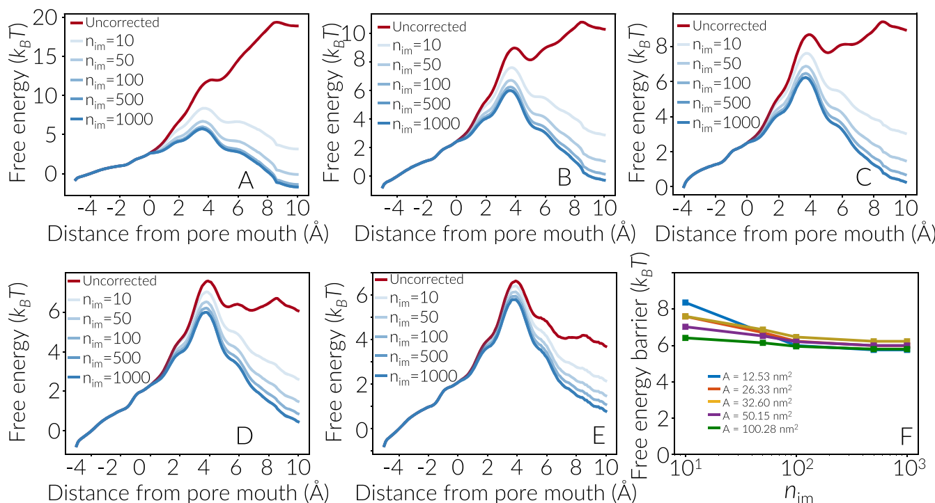
FIG. 5. The sensitivity of the ICDM correction to the number of image charges. Panels (a)–(e) illustrate the corrected profiles for systems with cross-sectional surface areas of (a) 12.53 nm 2 , (b) 26.33 nm 2 , (c) 32.60 nm 2 , (d) 50.15 nm 2 , and (e) 100.28 nm 2 , when different numbers of image charges are utilized. (f) The calculated translocation barriers for various systems as a function of n_{\text{im}} , indicating satisfactory consistency when more than 100 image charges are included. These calculations employ n_{\text{prd}} = 200 periodic replicates, equivalent to 400 replicates in each direction.
