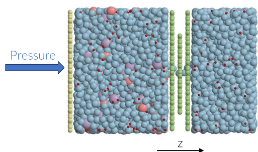
FIG. 3. A representative configuration of the system setup. A three-layer graphitic membrane separates a feed consisting of water, sodium, and chloride from a pure water filtrate. The system is enclosed in the z -direction by graphene pistons upon which a force can be exerted to generate a pressure gradient. The graphics have been prepared using injavis . 47
