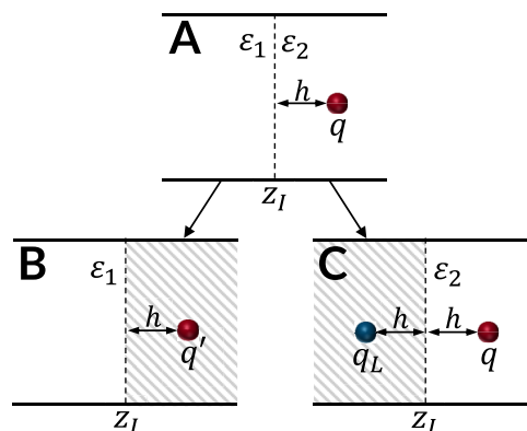
FIG. 1. Schematic representation of the application of the method of images to two adjacent dielectric regions with dielectric constants \epsilon_1 and \epsilon_2 . To accurately represent the actual charge distribution depicted in (a), where a point charge exists in region 2, surrogate charge configurations are devised for regions 1 (b) and 2 (c). In each panel, the solution of the Poisson equation within the white region is determined by the real charge(s) within that region along with the image charge(s) situated within the dashed region.
