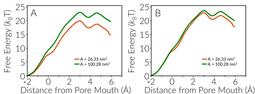
FIG. 9. (a) Uncorrected and (b) corrected free energy profiles for the F_{0,1} \rightarrow F_{1,1} transition. The correction has been applied using Eq. (27).
