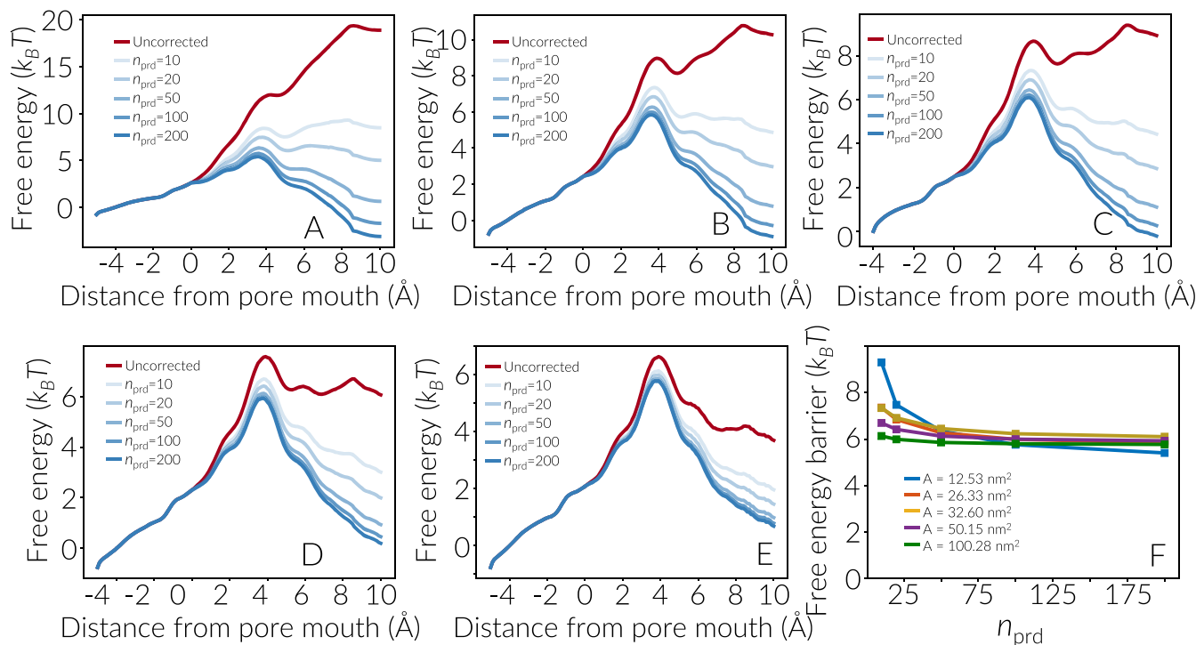
FIG. 6. The sensitivity of the ICDM correction to the number of periodic replicates. Panels (a)–(e) demonstrate corrected profiles for systems with cross-sectional surface areas of (a) 12.53 \text{nm}^2 , (b) 26.33 \text{nm}^2 , (c) 32.60 \text{nm}^2 , (d) 50.15 \text{nm}^2 , and (e) 100.28 \text{nm}^2 with different number of periodic replicates. (f) The calculated translocation barriers for various systems as a function of n_{\text{prd}} , indicating satisfactory consistency for n_{\text{prd}} \geq 50 . These calculations employ n_{\text{im}} = 1000 image charges.
