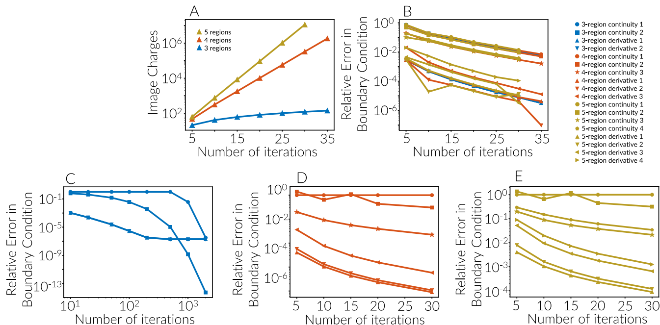
FIG. 10. (a) The total number of image charges as a function of the number of iterations in systems with m = 3, 4 , and 5 dielectric domains. (b) The convergence of Algorithm 1 when all regions have modest dielectric constants, namely, (\epsilon_1, \epsilon_2, \epsilon_3) = (20, 1, 20) , (\epsilon_1, \epsilon_2, \epsilon_3, \epsilon_4) = (20, 1, 10, 20) , and (\epsilon_1, \epsilon_2, \epsilon_3, \epsilon_4, \epsilon_5) = (20, 1, 10, 15, 20) for m = 3, 4 , and 5 , respectively. As can be noted, a reasonably small relative error is obtained for all boundary conditions after 35 iterations. (c)–(e) The convergence of the algorithm when \epsilon_1 = 2 \times 10^9 . The other dielectric constants are given by: (c) (\epsilon_2, \epsilon_3) = (1.16, 70.5) for m = 3 , (d) (\epsilon_2, \epsilon_3, \epsilon_4) = (1.16, 82, 70.5) for m = 4 , and (e) (\epsilon_2, \epsilon_3, \epsilon_4, \epsilon_5) = (1.16, 88.3, 82, 70.5) for m = 5 . Except for (c), the convergence at the conductor surface is not achieved even after including millions of image charges.
