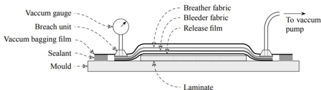
Figure 2. Vacuum Bagging Molding Process [26]. Reprinted with permission from Springer Nature.
