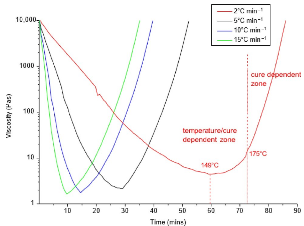
Figure 12. Resin viscosity as a function of heating rates [99].
