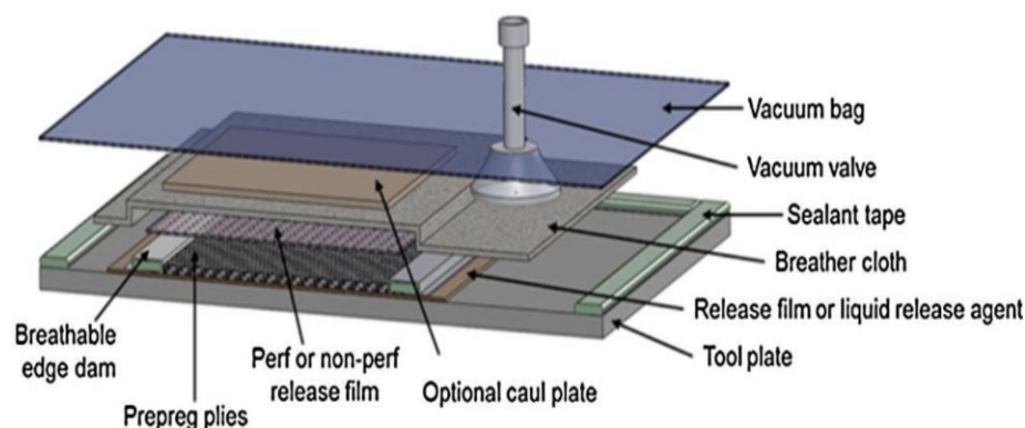
Figure 5. Manufacturing assembling of VBO cure [21]. Reprinted with permission from Elsevier.
