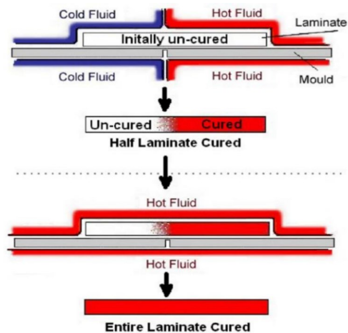
Figure 11. Schematics of the Molding Process [97]. Reprinted with permission from Elsevier.
