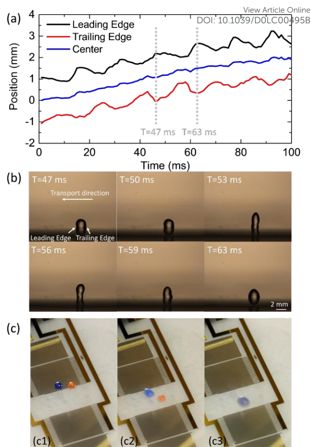
Fig. 3 Analysis of droplet movement on SAWN-ARC chips. (a) Droplet edge position change with time, modulated by the SAWN power. The average transport speed can be estimated from the center position change over 100 ms sampling time. (b) High-speed camera capture of droplet silhouettes (Movie S1). (c) Droplets moving and merging operation on SAWN platform with ARC tracks. (c1) Placement of colored droplets (blue and orange) on the two ARC tracks. (c2) Droplets moving along ARC actuated by SAW. (c3) Droplets stopping, merging and mixing at the central hydrophilic nebulization region.
