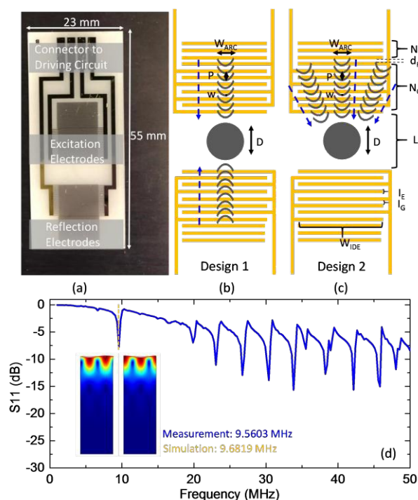
Fig. 1 SAWN chip design with ARC and frequency measurements. (a) Top view of the SAWN chip after dicing. (b) and (c) SAWN platform setup with ARC. Two designs of the ARC patterns for droplet movement control. Dotted blue arrows indicate the droplet movement direction. The grey arc-shaped rungs and center circle patterns are hydrophilic regions, treated with TMS. The other regions of the SAWN chip are covered with Cytop. (d) The S11 measurement result of the SAWN chip. The scanning start frequency is 1 MHz and the end frequency is 50 MHz. The inserts show the simulated transverse and longitudinal SAW modes at the lowest order resonance frequency, corresponding to the frequency at the ochre dotted line from the S11 curve. The general trend for S11 value decreases at higher frequencies, which could come from the resistive energy loss at the electrical connection.
