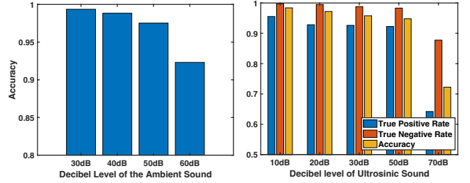
Fig. 18. Impact of ambient noise.
