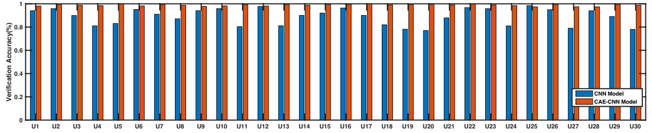
Fig. 10. User verification accuracy and the CNN vs. CAE-CNN comparison (standalone VR).
