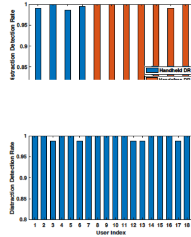
Fig. 13: Distraction detection performance for different users.
