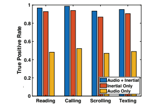
Fig. 21: Detailed performance of ture sets to recognize fine-grained handheld phone use.
