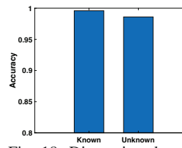
Fig. 18: Distraction detect unenrolled users (not in the train- ing model)
