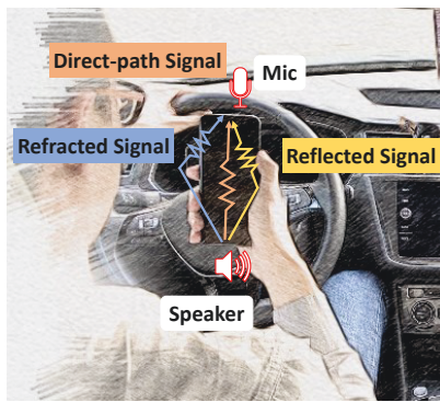
Fig. 1: Illustration of acoustic signal interaction with driver's hand.
