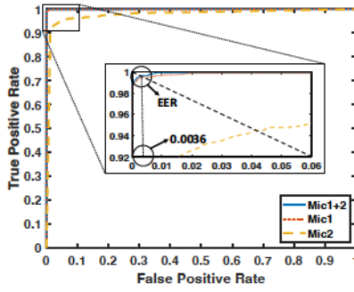
Fig. 11: Distracted detection performance of our system.
