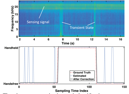
Fig. 6: The phone-use monitoring and classification error correction.
