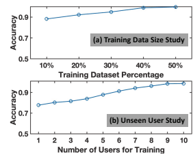
Fig. 19: Training data size and unseen user study performance
