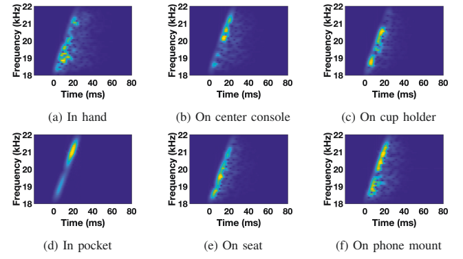
Fig. 5: Short-time Fourier transform of different phone use statuses.
