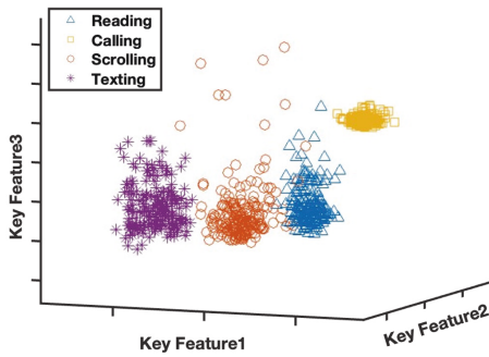
Fig. 9: Using cross-domain features to recognize fine-grained handheld phone use.
