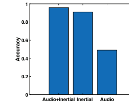
Fig. 20: Using different rea- ture sets to recognize fine-grained handheld phone use.
