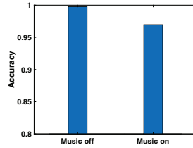
Fig. 17: Impact of in-car music for phone distraction detection.
