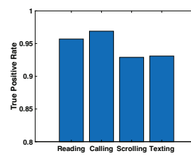
Fig. 26: Fine-grained phone-use recognition monitoring.
