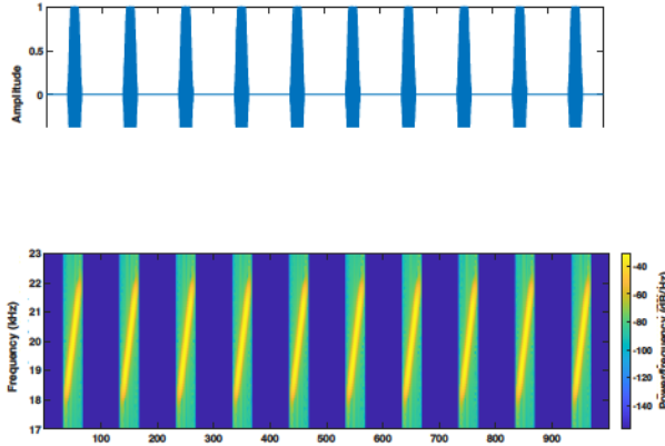
Fig. 3: The periodic ultrasonic pulse signals for sensing.
