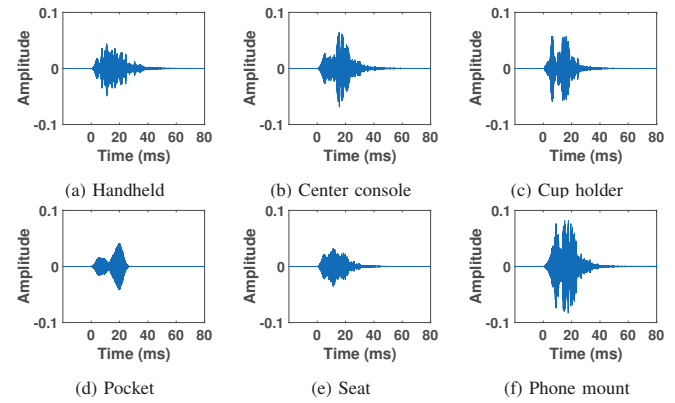
Fig. 2: Acoustic response of different phone placement.
