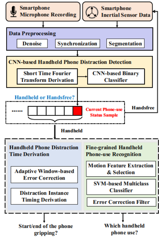
Fig. 4: The architecture of our system.
