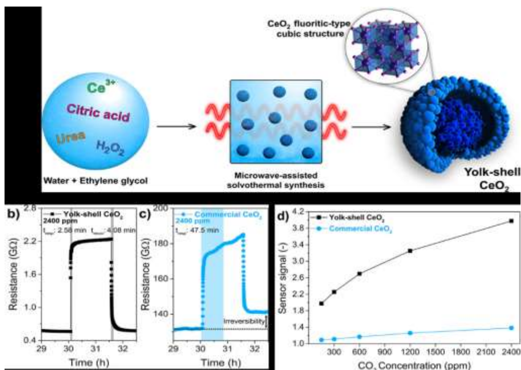
Figure 24. Microwave-assisted solvothermal synthesis of yolk-shell CeNPs (a), response and recovery times to 2400 ppm of the sensor prepaid with yolk-shell CeNPs (b) as compared to the commercial CeNPs (c), and comparative sensor signal in response to CO 2 concentrations (d) (Reprinted with permission from Ref 411 . Copyright 2020 American Chemical Society).
