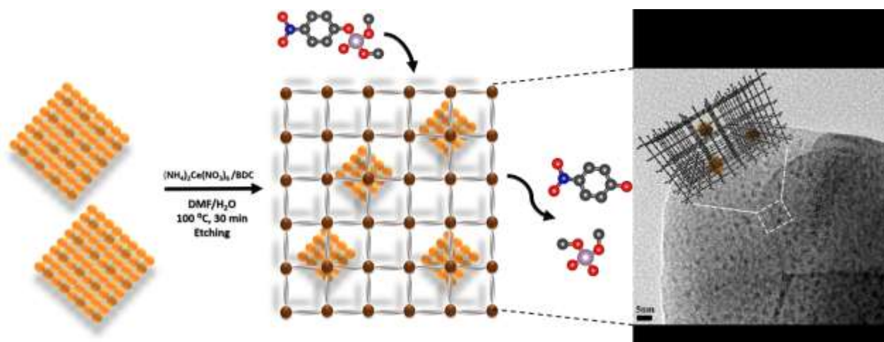
Figure 20. Schematic of CeNPs immobilization inside Ce-MOF for DMNP degradation and the subsequent CeNP –MOF structure analysed by TEM (Reprinted with permission from Ref 300 . Copyright 2020 American Chemical Society).
