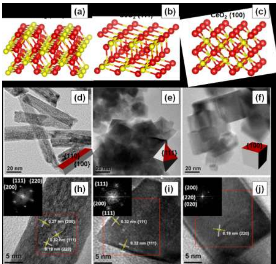
Figure 4. Atomic structures of the three low index crystal planes of ceria. (a) 110 (b) 111 and (c) 100. Red and yellow colored spheres represent \text{O}^{2-} and \text{Ce}^{4+} ions, respectively. TEM and HRTEM images of the three different ceria nanoshapes (d, h) nanorods, (e, i) nanooctahedra and (f, j) nanocubes. Fourier transform patterns of selected areas of the samples are shown in the insets of HRTEM images. Figures 4d-j reprinted with permission from Ref 39 . Copyright 2018 American Chemical Society.
