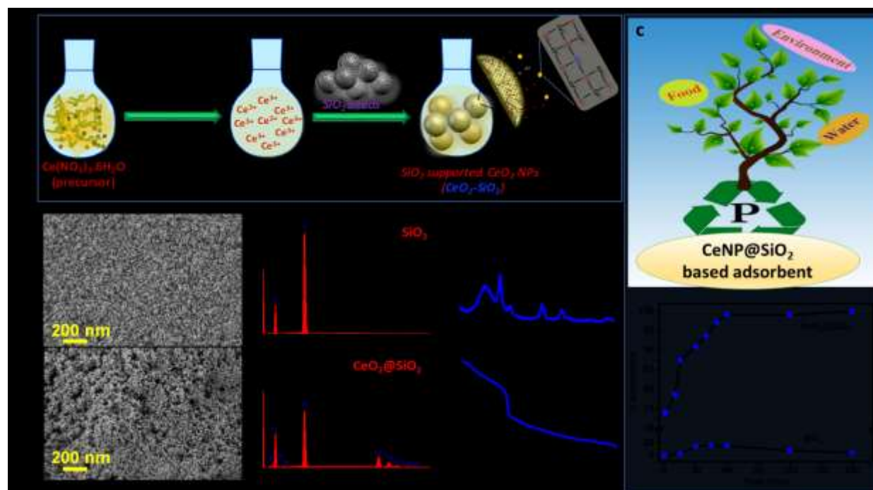
Figure 33. Synthesis of \text{CeO}_2@\text{SiO}_2 adsorbent (a) with SEM, XRD and TGA characterization (b) and adsorption isotherms for the removal of phosphate (c) showing significantly enhanced adsorption capacity of the for \text{CeO}_2@\text{SiO}_2 as compared to \text{SiO}_2 (Reprinted with permission from Refs 459 . Copyright 2019 American Chemical Society.).
