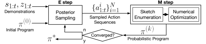
Fig. 1: Overview of PLUNDER
