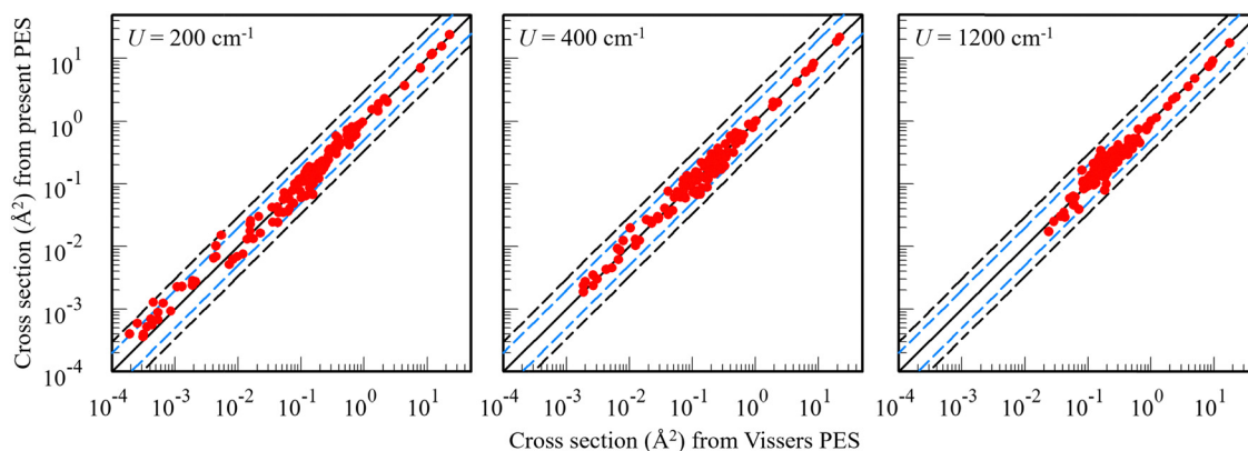
Fig. 7 Comparison of MQCT state-to-state transition cross sections for CO + CO system obtained using the present PES and Vissers et al. PES for three values of collision energy U (indicated in each frame). The initial state was (j_1 j_2) = (0, 0) . Blue dashed lines represent a factor of 2 difference and black dashed lines represent a factor of 3 difference.
