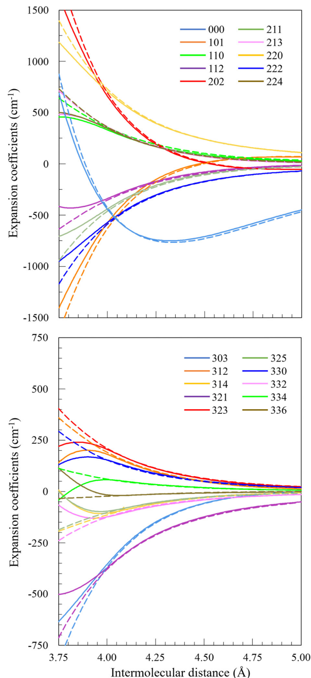
Fig. 5 Radial dependence of 20 expansion coefficients v_{\lambda_1\lambda_2\lambda}(R) for two CO + CO PESs in the interaction region: This work (solid line) and Visser et al. (dashed line). Colors correspond to different sets of \lambda_1\lambda_2\lambda , as indicated.
