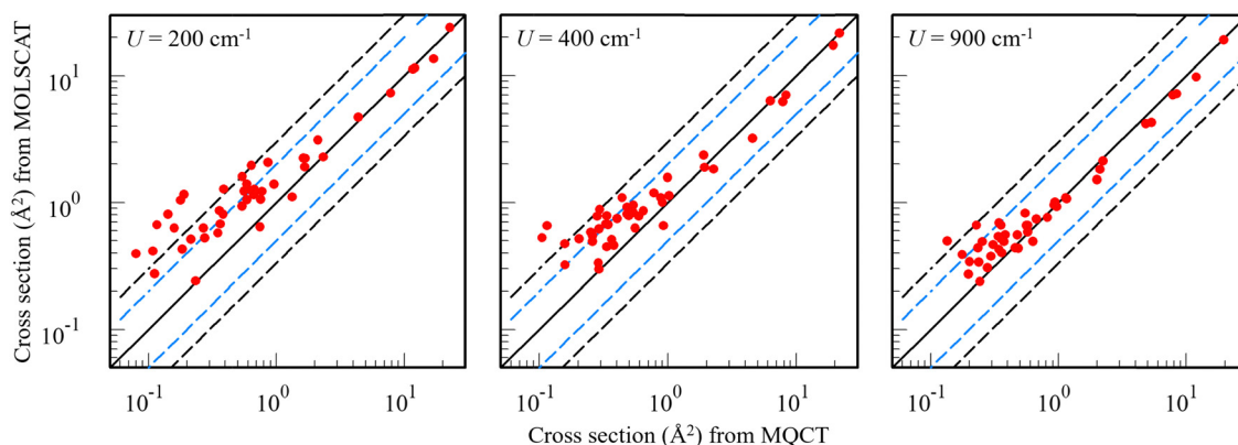
Fig. 8 Comparison of MQCT and MOLSCAT state-to-state transition cross sections for CO + CO system obtained using Vissers et al. PES. The initial state was (j_1 j_2) = (0, 0) ; the final states are those reported in ref. 19 with all combinations of j_1 \leq 8 and j_2 \leq 8 . Blue dashed lines represent a factor of 2 difference and black dashed lines represent a factor of 3 difference.
