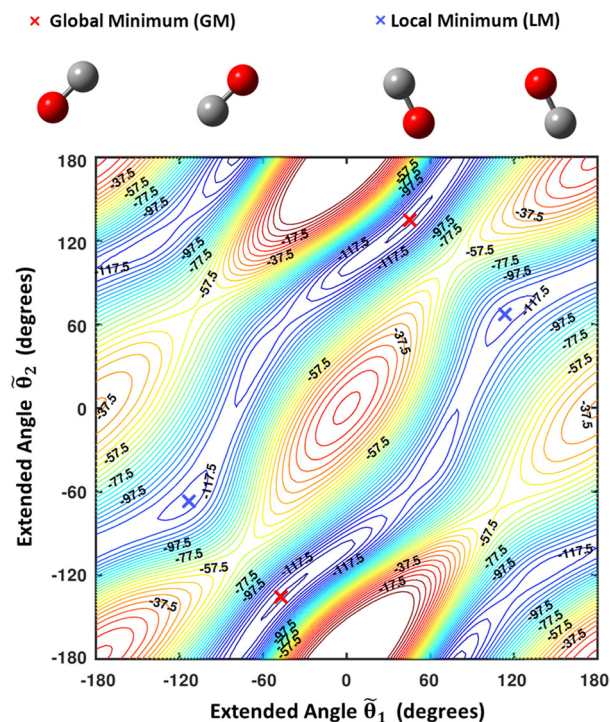
Fig. 2 R -optimized contour plot of the PES as a function of the extended angles \tilde{\theta}_1 and \tilde{\theta}_2 for planar configurations. For each pair of angles, the energy (given in \text{cm}^{-1} ) is optimized with respect to the center-of-mass distance R . See the text for details.
