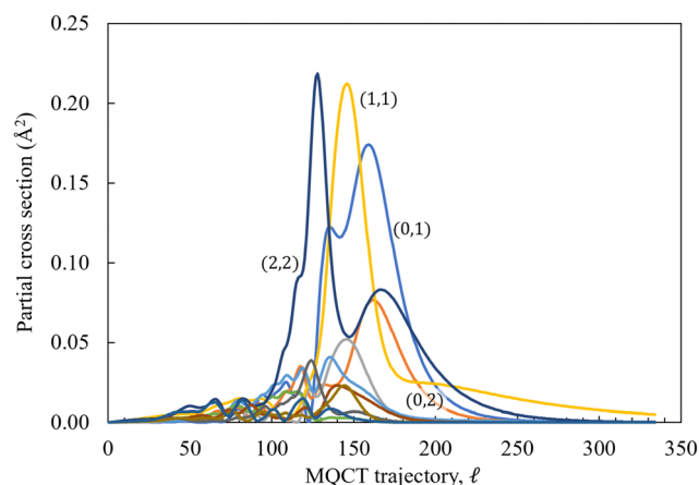
Fig. 4 Partial cross sections for excitation of various states in CO + CO collision at 1200 cm -1 . The initial state is (0,0). Final states ( j_1j_2 ) are indicated for the 4 most intense transitions. The PES of Visser et al. was used for these tests.
