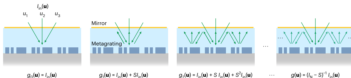
Fig. 1 | Si metagrating-based integral equation solver. An input vector \mathbf{I}_{\text{in}} is fed to the system in the form of N plane waves with different complex amplitudes incident along N diffraction channels. The signal interacts repeatedly with a metagrating, bouncing back from a partially reflecting mirror, each time multiplied by the metagrating scattering matrix and therefore building up the
