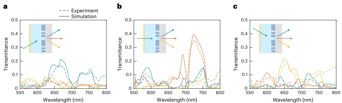
Fig. 5 | Optical characterization of S_{27} . a–c, Experimental (dashed lines) and simulated (solid lines) transmittance spectra of the completed metastructure. Insets show a schematic visualization of the metastructure indicating the
