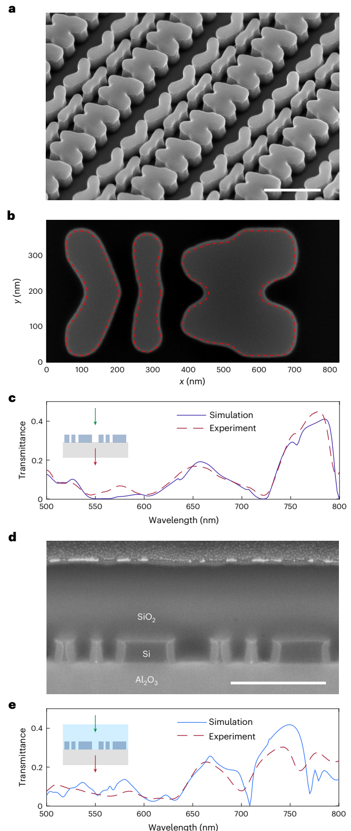
Fig. 4 | Fabrication and optical characterization of the optical analogue integral equation solver. a, Tilted scanning electron microscopy (SEM) image of the patterned Si metagrating. Scale bar, 500 nm. b, Zoomed-in top-view SEM image of a single unit cell compared with the desired optimized contour (red dashed line). c, Experimental (dashed red line) and simulated (dark blue line) transmittance spectra of the metagrating after the Si etch step (that is, without silica spacer and top mirror). The sample was illuminated under normal incidence (green arrow) and the transmitted zeroth-order diffraction intensity was collected (red arrow, inset) as a function of incident wavelength. d, SEM image of a focused-ion-beam-milled cross-section of the same metagrating embedded in a SiO 2 spacer. Scale bar, 500 nm. e, Experimental (dashed red line) and simulated (blue line) transmittance spectra of the metagrating after the SiO 2 planarization step. The input polarization is TE for c and e.
