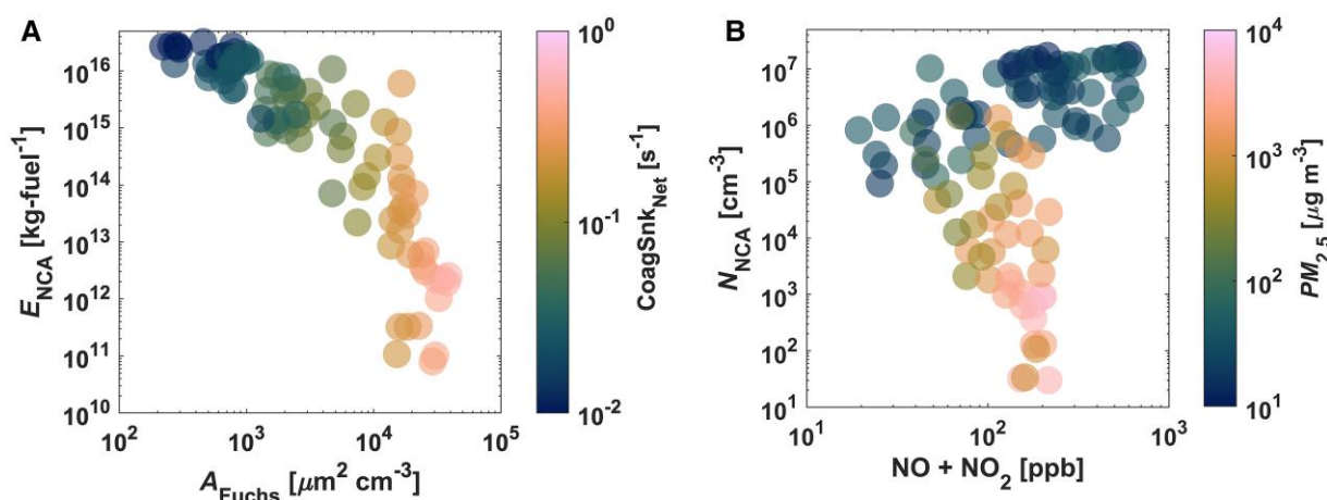
Fig. 2. Dynamics of combustion-derived NCA in the indoor atmospheric environment during gas cooking. A) Relationship between the propane-gas-cooking-emitted NCA emission factor ( E_{NCA} ) and coagulation scavenging parameters, the aerosol Fuchs surface area ( A_{Fuchs} ) and net coagulation sink ( \text{CoagSnk}_{Net} ), during the gas-stove-combustion period. The color of the markers represents \text{CoagSnk}_{Net} . B) Relationship between size-integrated (1.18–3 nm) propane-gas-cooking-emitted NCA number concentrations ( N_{NCA} ) and conventional indoor air pollution markers, \text{PM}_{2.5} mass concentrations, and \text{NO} + \text{NO}_2 mixing ratios, during the gas-stove-combustion period. The color of the markers represents the \text{PM}_{2.5} mass concentrations.
