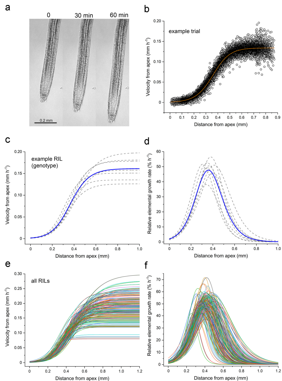
Figure 1. Overview of kinematic data collection starting with example images of roots and ending with a population of velocity and relative elemental growth rate profiles obtained from Cvi × Ler recombinant inbred lines. (a) Three images selected from the beginning, middle, and end of a typical 120-frame trial. (b) Velocity point cloud showing the spatial distribution of displacement velocities of one root
