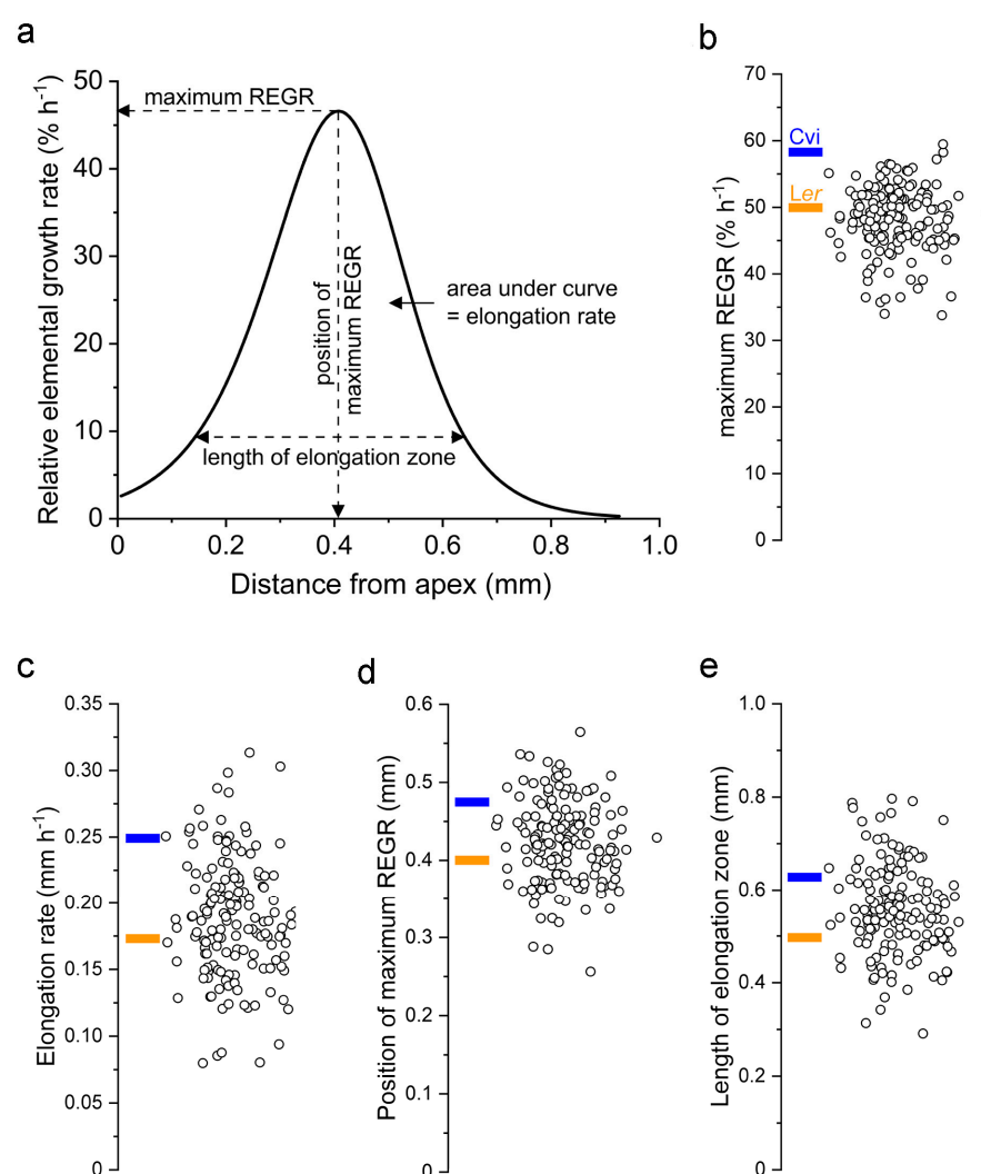
Figure 2. Kinematic traits of the root elongation zone and their variation across the Cvi \times Ler RIL population. (a) A representative relative elemental growth rate (REGR) curve labeled with the four kinematic traits of the elongation zone studied here. (b) The values of maximum REGR obtained for the RIL population. The blue and orange bars indicate the mean value of the inbred parents. (c) Same as (b) but for elongation rate. (d) Position of maximum REGR. (e) Length of elongation zone.
