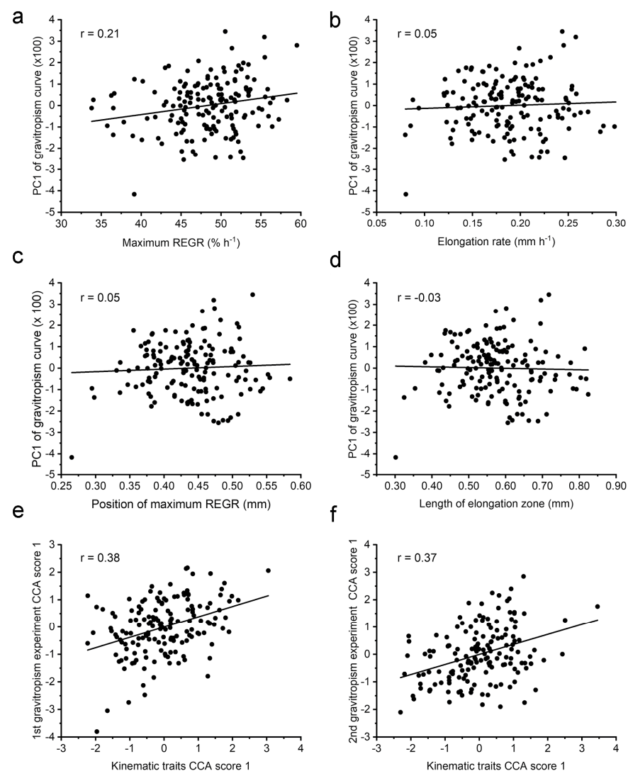
Figure 6. Correlations between each elongation zone trait and PC1 of gravitropism curves, and a canonical correlation analysis between all elongation zone traits and gravitropism data. (a) Gravitropism versus maximum REGR; (b) gravitropism versus elongation rate; (c) gravitropism versus position of maximum REGR; (d) gravitropism versus length of elongation zone; (e) canonical correlation analysis (CCA) score of the 1st gravitropism experiment versus the same for the set of four elongation zone traits; (f) same as (e) except the gravitropism data came from a second gravitropism trial.
