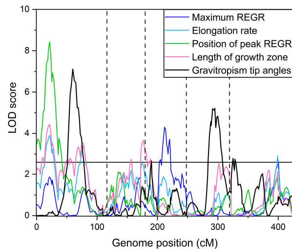
Figure 5. QTL map of the four elongation zone (kinematic) traits and tip angle during gravitropism from a previously published study [17]. The tip angle data represent the 4 h point of an 8 h time course. The QTL intervals for elongation zone traits overlap very little with the gravitropism QTL intervals.
