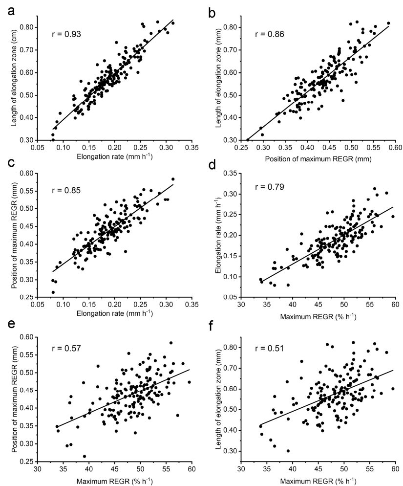
Figure 4. Correlation of each possible combination of four kinematic traits and the r value determined by a linear fit. (a) Length of elongation zone versus elongation rate. (b) Length of elongation zone versus position of maximum REGR. (c) Position of maximum REGR versus elongation rate. (d) Elongation rate versus maximum REGR. (e) Position of maximum REGR versus maximum REGR. (f) Length of elongation zone versus maximum REGR.
