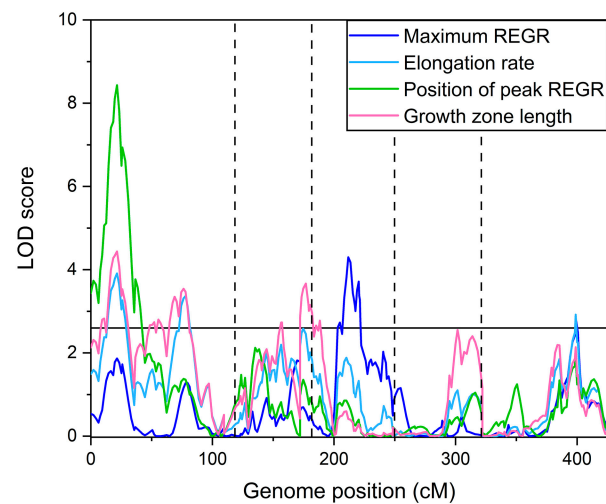
Figure 3. QTL map for each of the four kinematic traits of the elongation zone. The horizontal line is a significance threshold determined by the permutation method. The vertical dashed lines denote the boundaries of the five chromosomes.
