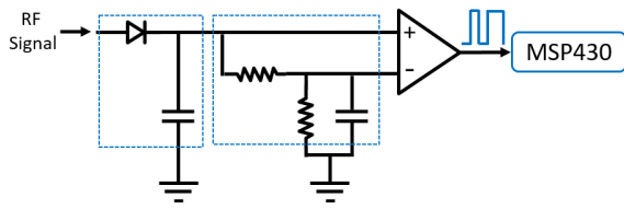
Figure 4: Low-power down-link receiver circuit diagram.
