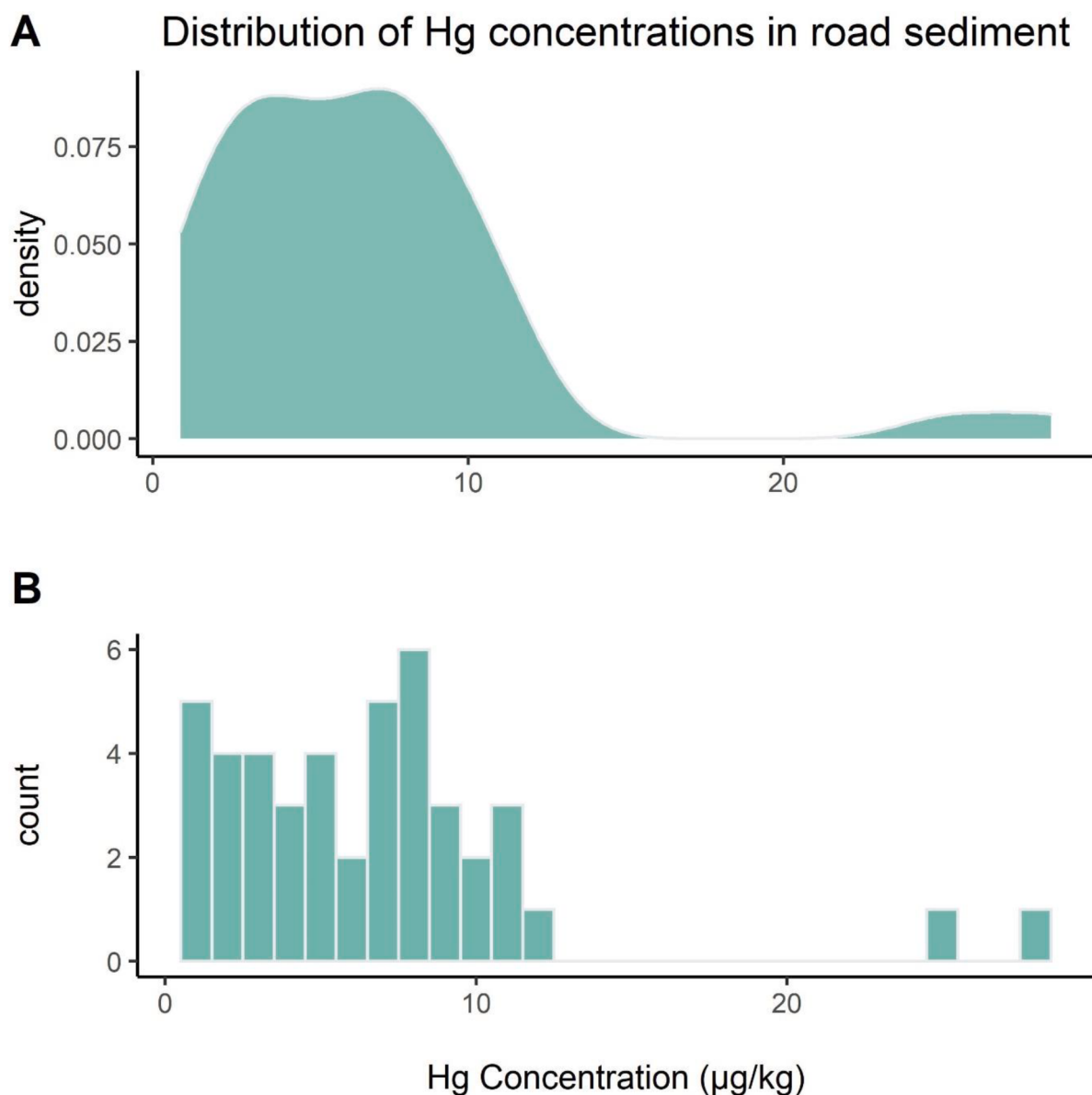
Fig. 2. Smoothed kernel density estimate (A) and histogram (B) showing the distribution of concentrations of Hg in road sediment samples in \mu\text{g/kg} .
