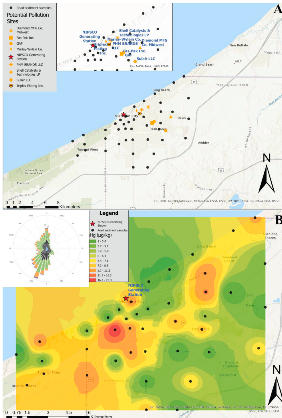
Fig. 3. Maps of: (A) Sampling locations and potential pollutant sites, including the NIPSCO generating plant and (B) Inverse distance weighted (IDW) map of Hg concentrations (in \mu\text{g/kg} ) with the wind rose diagram for the area (National Oceanic and Atmospheric Administration (NOAA), 2023).
