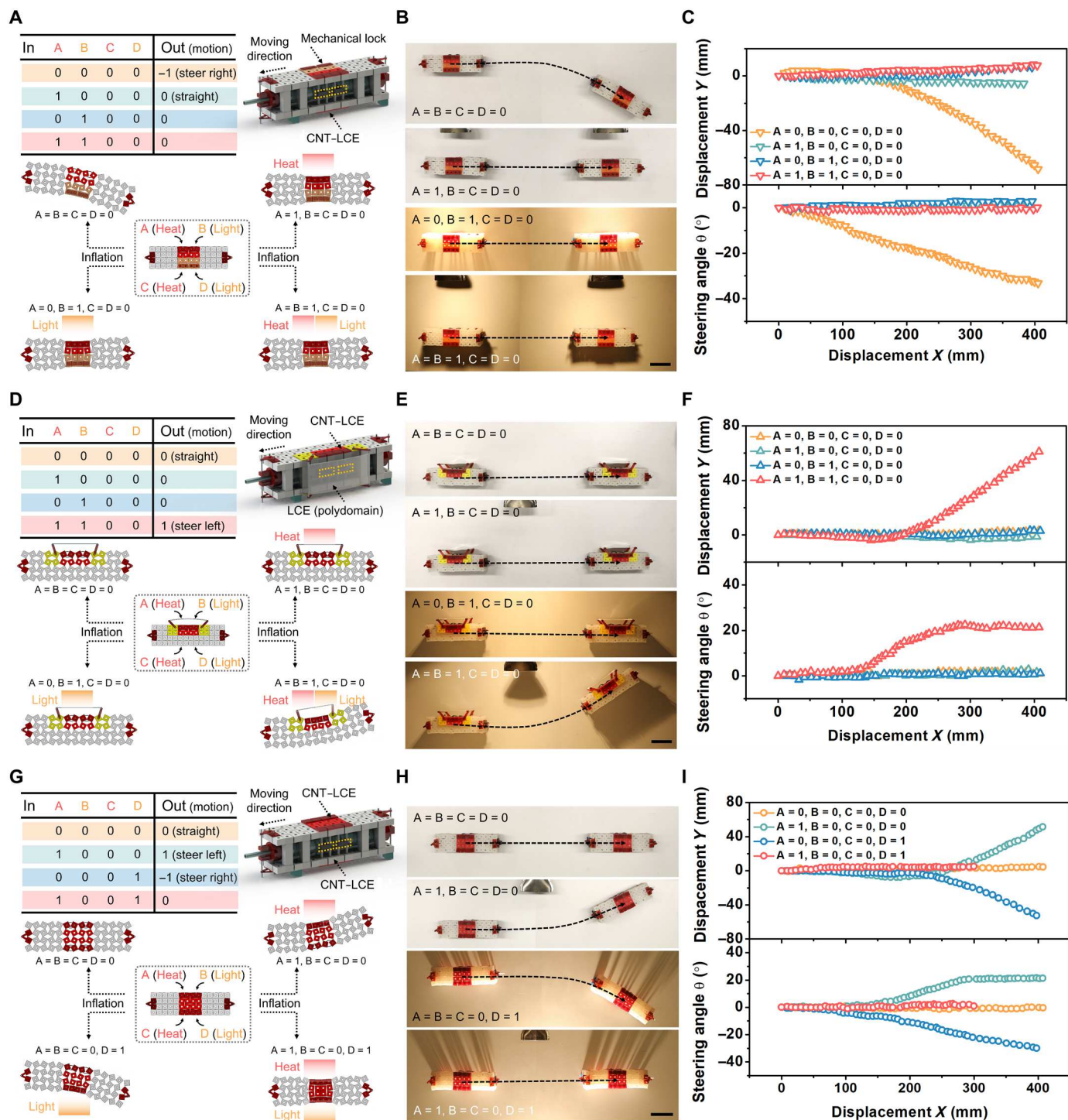
Fig. 5. Embodying distributed, multistimuli-responsive logic via interaction of multiple control modules. Interactions of multiple control modules can be complex (see complete truth tables in fig. S31). Here are a few simplified examples: (A) The combination of a “mechanical lock” control module and the CNT-LCE module of Fig. 3C causes the robot’s steering to obey a NOR response. (B and C) Experimental images and trajectories, respectively, of the robot with different heat/light inputs. (D) In another example, a “mask” control module is used in conjunction with the CNT-LCE module of Fig. 3C to steer in accordance with an AND strategy [for the environment shown in (E)]. (E and F) Experimental images and trajectories, respectively, of the robot with different heat/light inputs. (G) In another example, two identical control modules (actuated by heat or light) are distributed symmetrically along the two sides of the robot body, which enable the robot to realize XOR response. (H and I) Experimental images and trajectories, respectively, of the robot with different heat/light inputs. Scale bars (B), (E), and (H), 5 cm.
