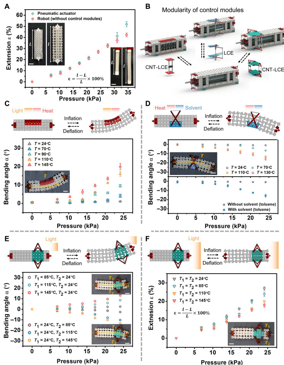
Fig. 3. Physical shape changes of soft autonomous robots in response to environmental inputs. (A) The extension ratio \epsilon of the pneumatic actuator and the robot (without any control modules) as a function of applied pressure. (B) Multiple types of modular control units are developed. They can be easily attached to or removed from the body of the robot. (C) As one example, a control module can sense and respond to heat or light. (D) In this example, a different control module design causes the robot to bend away from heat or solvents. (E and F) In another example, a control module is designed to bend the robot so that its end will align toward a light. Scale bars (A), (C), (D), (E) and (F), 2 cm.
