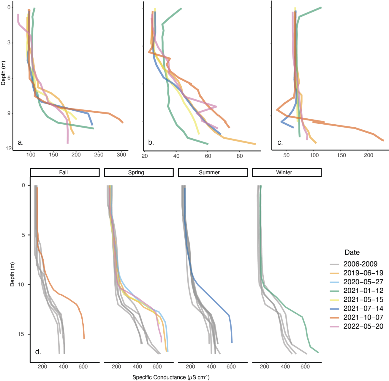
Figure 3. Specific conductance profiles of a) Arco Lake, b) Budd Lake, c) Josephine Lake, and d) Deming Lake. For
