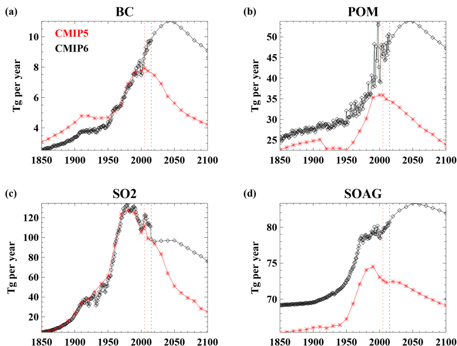
Figure 1. Emissions of global anthropogenic and biomass burning emissions, including (a) black carbon (BC), (b) primary organic matter (POM), (c) sulfur dioxide, and (d) gas-phase condensable sources of secondary organic aerosols (SOAGs) for CMIP5 (red) and CMIP6 (black) forcings.
