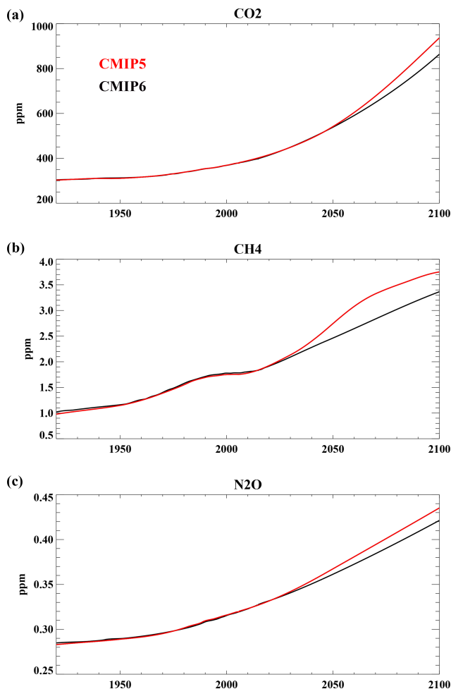
Figure 3. Prescribed concentrations of greenhouse gases, including (a) \text{CO}_2 , (b) \text{CH}_4 , and (c) \text{N}_2\text{O} for CMIP5 (red) and CMIP6 (black) forcings.
