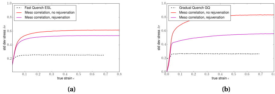
Figure 7. Evolution of the standard deviation of the internal stress field in the glasses (a) ESL and (b) GQ vs meso model.
