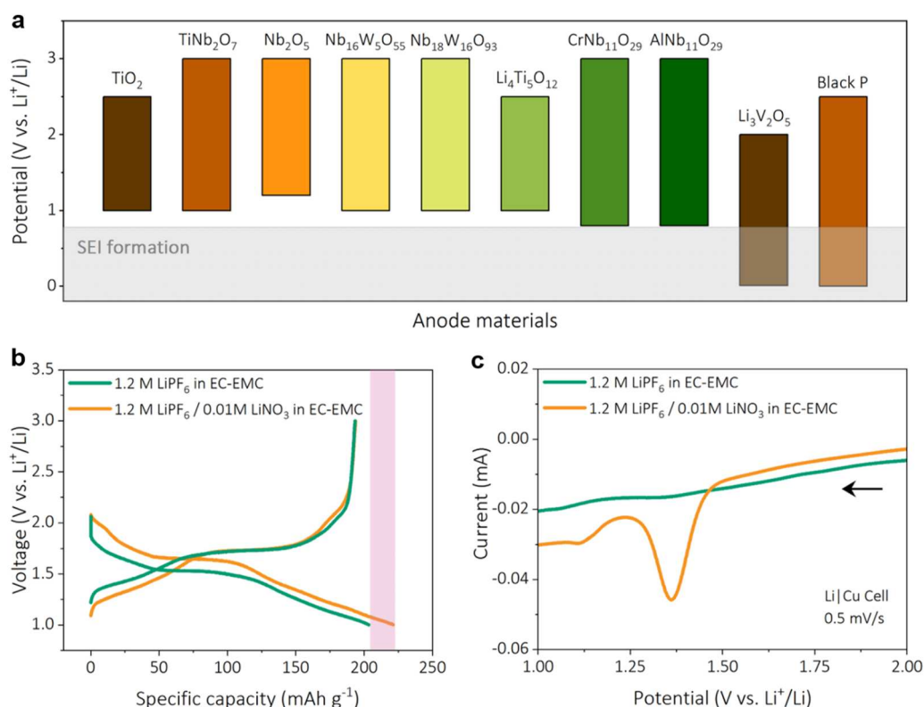
Fig. 1 Design of SEI layers on \text{H-Nb}_2\text{O}_5 . (a) Operating potential (vs. \text{Li}^+/\text{Li} ) range of typical anode materials capable of fast-charging, based on previous reports. 9–14,22,23,35 (b) Initial charge and discharge (C/4 rate) curves for \text{H-Nb}_2\text{O}_5 with neat EC-based electrolyte and \text{LiNO}_3 -added EC-based electrolyte. (c) Linear sweep voltammetry ( 0.5 \text{ mV s}^{-1} ) of \text{Li}|\text{Cu} cells with neat EC-based electrolyte and \text{LiNO}_3 added EC-based electrolyte, indicating SEI formation with \text{LiNO}_3 decomposition.
