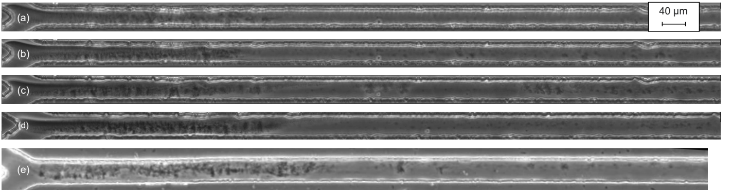
Figure 7: Microscopy images of different deposition events obtained from different devices and conditions. Images (a), (b), (c), and (d) show clogs formed at flow rates Q_T = 1.2, 2.4, 6.0, and 12.0 \mu\text{L/min} , respectively. Microscopy shows little difference at these different flow rates. (e) Smoother channel walls result in similar features in the gel deposit, regardless of the micron scale roughness.
