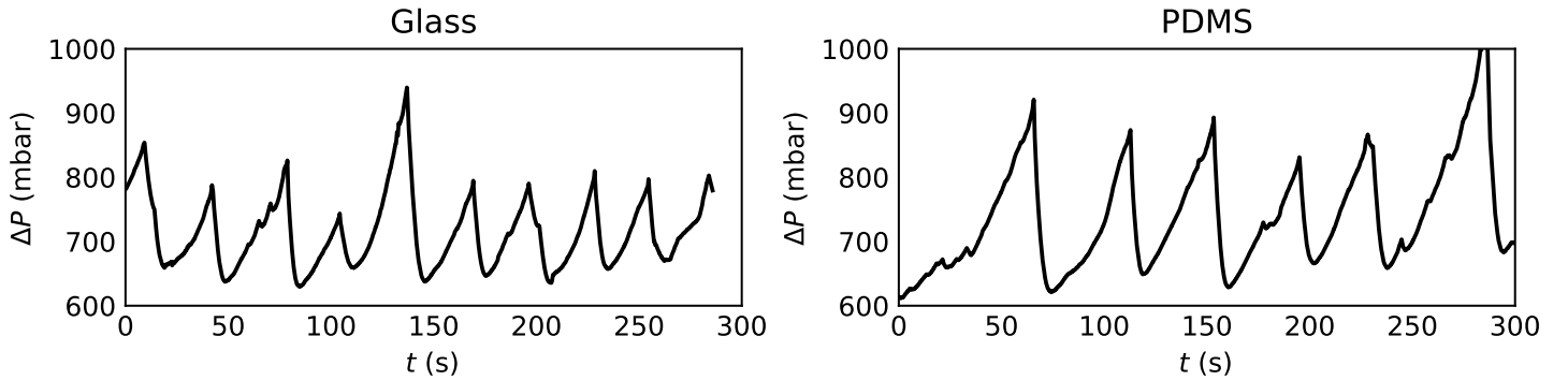
Figure 4: Traces of \Delta P(t) for flow through Y-shaped junctions made of PDMS adhered to glass slides with and without a PDMS coating exhibit similar intermittent flow behavior. This demonstrates that alginate gel clogging is not specific to glass or PDMS. Data is taken at C_{Alg} = 0.1\text{ mg/mL} , C_{Ca^{2+}} = 100\text{ mM} , Q_T = 12.0\mu\text{L/min} .
