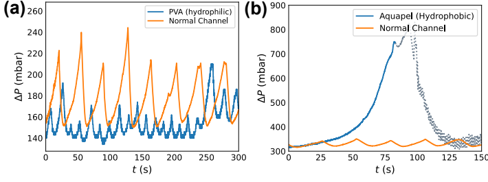
Figure 5: Traces of \Delta P(t) for flow through (a) a hydrophilic PVA-coated channel or (b) a hydrophobically coated channel show changes in feature size versus a channel with no coating. Alginate adheres more strongly to hydrophobic channels, although alginate deposition is seen in all cases. Data is taken at C_{Alg} = 0.1 mg/mL, C_{Ca^{2+}} = 100 mM. For (a) Q_T = 2.4 \mu\text{L}/\text{min} . while for (b) Q_T = 6.0 \mu\text{L}/\text{min} . Note: Aquapel coating interferes with the adhesion between the PDMS and glass. As a result, the channel delaminated at \tilde{80} seconds. Data after delamination is plotted as a dotted line.
