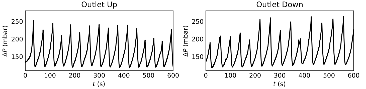
Figure 9: The plots show the behavior of intermittent flow when a device is oriented in the upright direction, with flow driven either against (‘Outlet Up’) or with (‘Outlet Down’) gravity. The flow behavior is the same in both cases, demonstrating that gravity is not a significant force for gel deposition. Data is taken at C_{Alg} = 0.1 mg/mL, C_{Ca^{2+}} = 100 mM and Q_T = 1.2\mu\text{L}/\text{min} .
