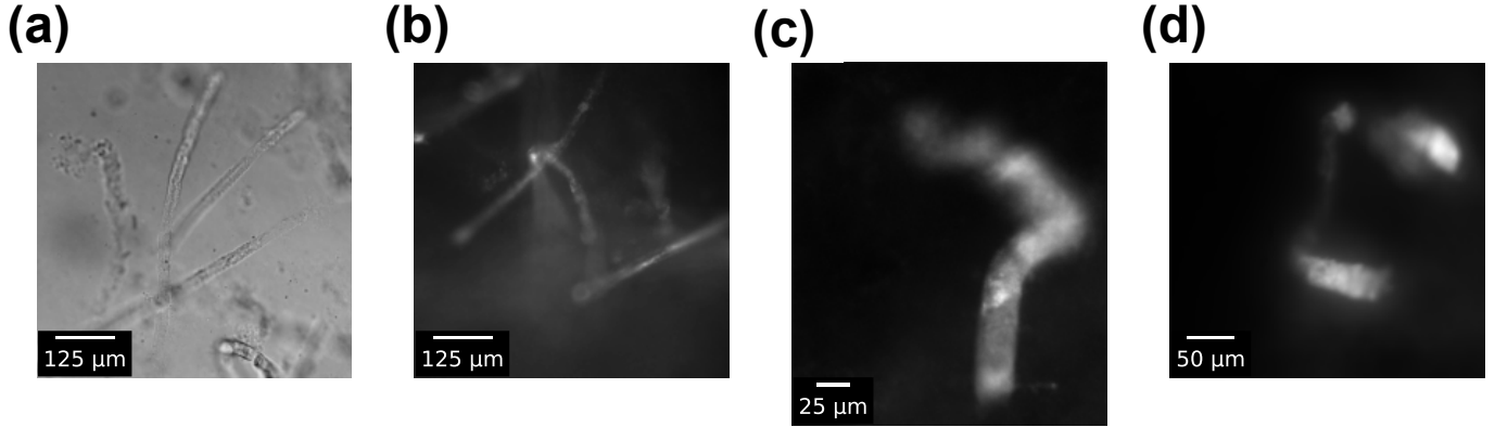
Figure 10: Additional microscopic images of eluted rods. Image (a) was taken using phase contrast microscopy, while images (b-c) use fluorescent microscopy to image embedded fluorescent particles. Images (a) and (b) were taken at 5x magnification and each show several rods that have not been separated from the eluted solution. Images (c) and (d) each show a single rod taken at 20x magnification.
