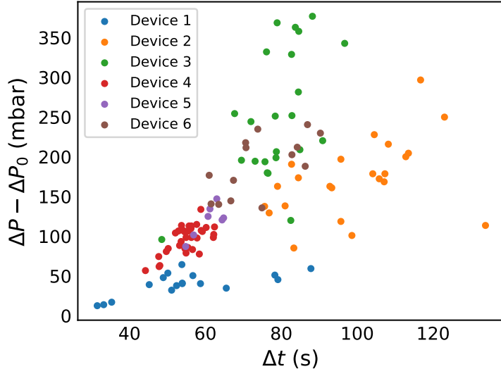
Figure 2: Device-to-device variation: The difference between the driving pressure at the point of greatest occlusion baseline pressure is plotted as a function of the time interval between ablation events. Each data point represents a single ablation event. Each color represents a separate device of the same design. Comparison of results from six different devices shows that replicate devices result in slightly different deposition/ablation patterns. Data is taken at C_{Alg} = 0.1\text{mg/mL} , C_{Ca^{2+}} = 100\text{mM} , Q_T = 1.2\mu\text{L/min} .
