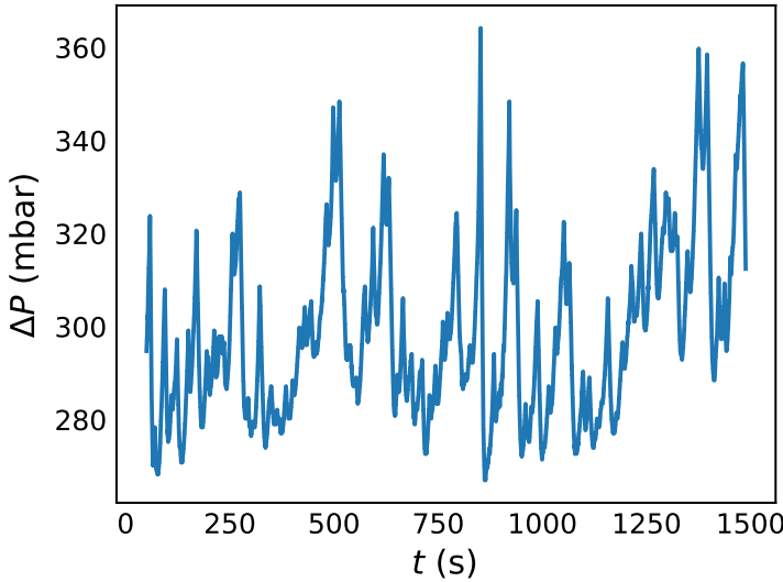
Figure 12: Intermittent deposition behavior is seen in alginate flows crosslinked by high concentrations of calcium, provided the flow rate is sufficiently high. The plot of \Delta P(t) represents data taken at C_{Alg} = 10 mg/mL, C_{Ca^{2+}} = 20 mM and Q_T = 6.0 \mu\text{L}/\text{min} .
