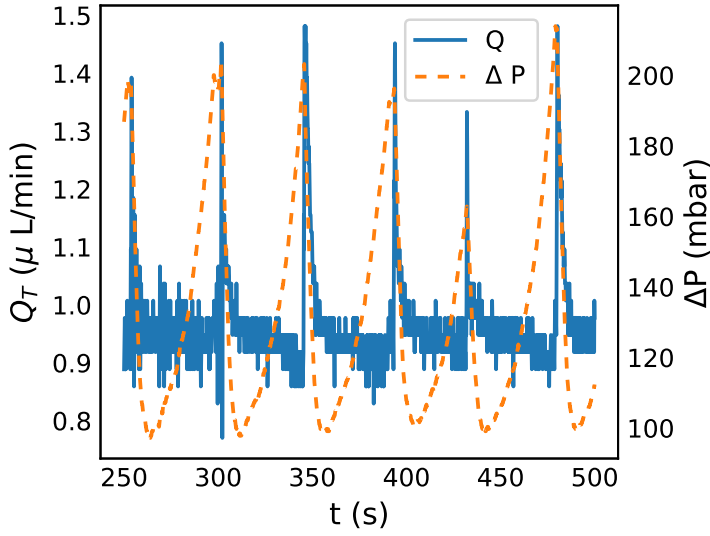
Figure 6: Flow rate varies slightly during clog ablation events. Several seconds are required for the pump to adjust to the decreased flow resistance as a gel clot is removed from the wall and exits the device. However, the magnitude and duration of the flow rate change are small compared to the magnitude in the pressure drop associated with alginate deposition. Q_T(t) is plotted in blue and \Delta P(t) in orange for data taken at C_{Alg} = 0.1 mg/mL, C_{Ca^{2+}} = 100 mM and Q_T = 1.2 \mu\text{L/min} .
