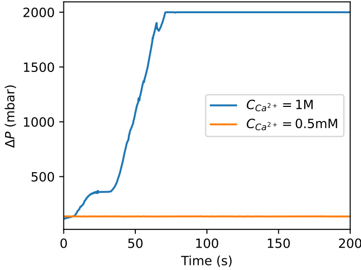
Figure 11: At high concentrations of calcium, complete clogging of the channel occurs at Q_T = 1.2 \mu\text{L}/\text{min} and C_{Alg} = 1 mg/mL, as shown in blue, when C_{Ca^{2+}} = 1000 mM. No deposition is seen, however, when the calcium concentration is low, C_{Ca^{2+}} = 0.5 mM, as seen in orange.
