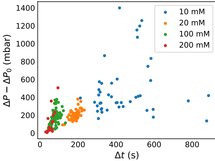
Figure 3: Variation between reaction conditions: The difference between the driving pressure at the point of greatest occlusion baseline pressure is plotted as a function of the time interval between ablation events. Four different calcium concentrations are shown, with fixed C_{Alg} = 0.1\text{mg/mL} and Q_T = 1.2\mu\text{L/min} . All data from SI Fig. 2 are plotted in green. The difference between conditions is larger than the difference between devices.
