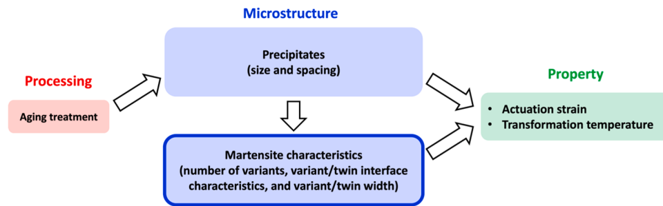
Fig. 10. The schematic highlighting the role of martensite variant number and boundary type in the processing-microstructure-property relationship of the \text{Ni}_{50.3}\text{Ti}_{29.7}\text{Hf}_{20} HTSMA.
