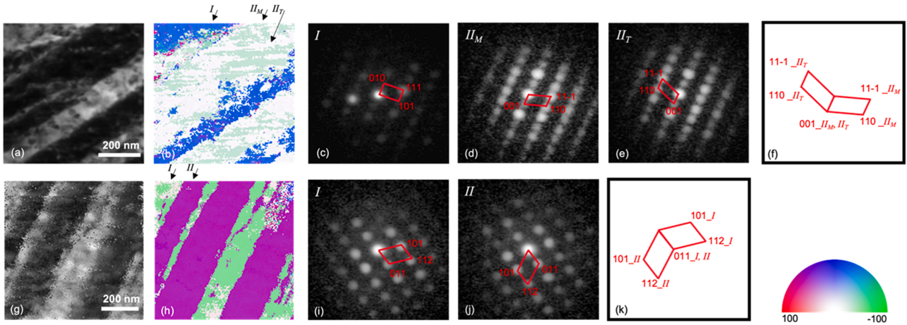
Fig. 5. (a) Virtual dark-field image of the 600 °C 10 h sample showing a number of martensite plates. (b) The corresponding orientation map. (c–e) Diffraction patterns from variant I, II M and II T in the orientation map. (f) Comparison between parallelograms from the diffraction pattern of variant II M and II T in the orientation map, showing the orientation relationship between them. Red parallelograms are used to demonstrate the symmetry of each diffraction pattern. (g–k) correspond to (a–f) but in a different area of the specimen to highlight the consistency and repeatability of the variant numbers and the orientation relationship between the martensite plates.
