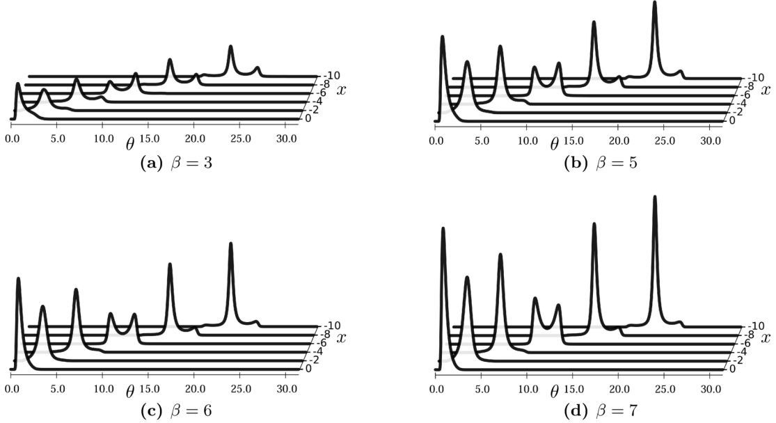
Figure 10. The evolution of \rho(x, \theta) := \frac{\partial H}{\partial \theta} as x decreases from x = 0 to -10 with step size \Delta x = -10^{-3} for \beta = 3, 5, 6, 7 . Finite-difference discretization with trapezoidal method is used on (2.11) with \Delta x = -10^{-3} and M = 10^4 for \theta \in [0, 10\pi] .
