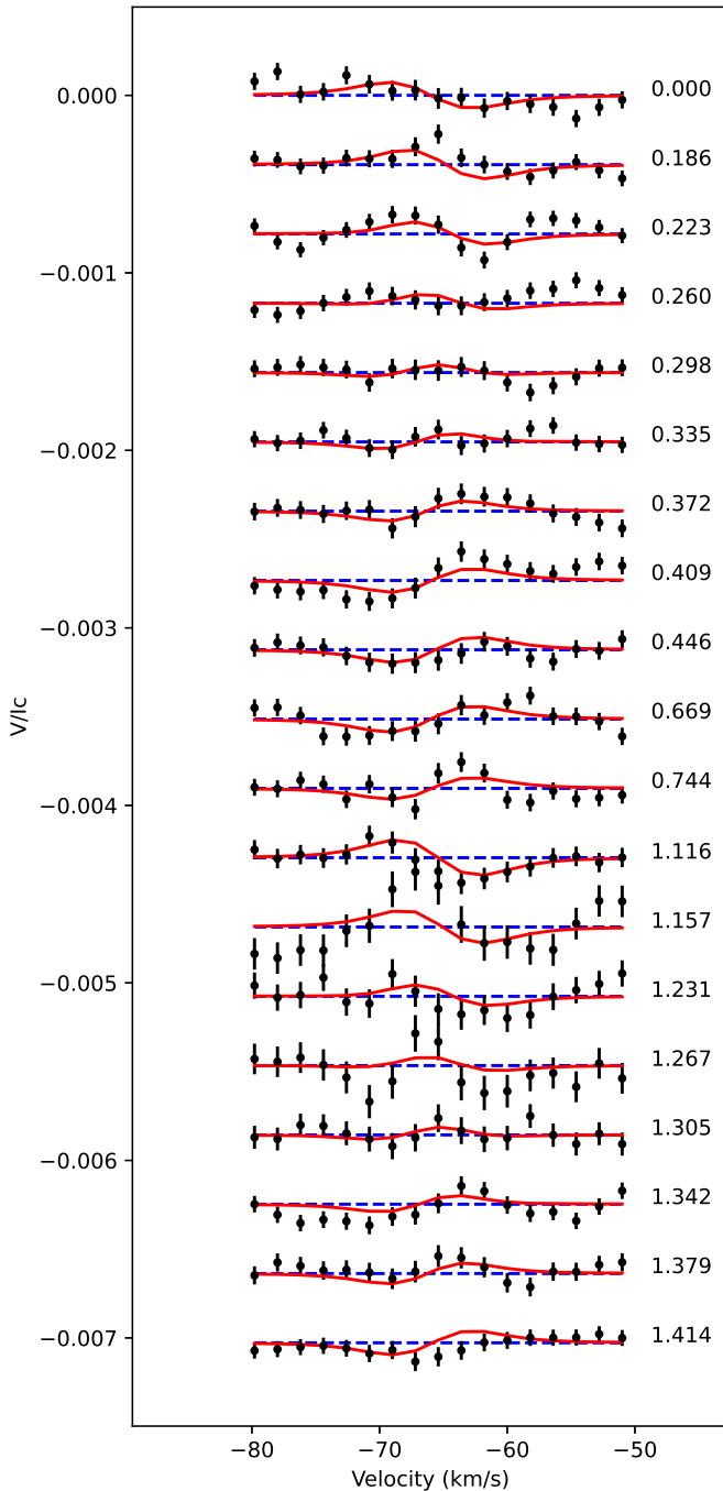
Figure 6. Stokes V LSD profiles obtained with Neo-NARVAL (black dots) and synthetic profiles produced by ZDI (red curves). Successive observations are vertically shifted for clarity, and the rotational phase \Phi of the observation is listed along the right side.
