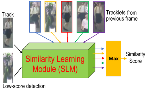
Figure 7: Appearance similarity between low-score detection at the current frame and tracks at the previous frame. Five tracklets compute a similarity score with the low-score detection using SLM. The most similar tracklet is selected, as indicated by the orange arrow in the figure.
