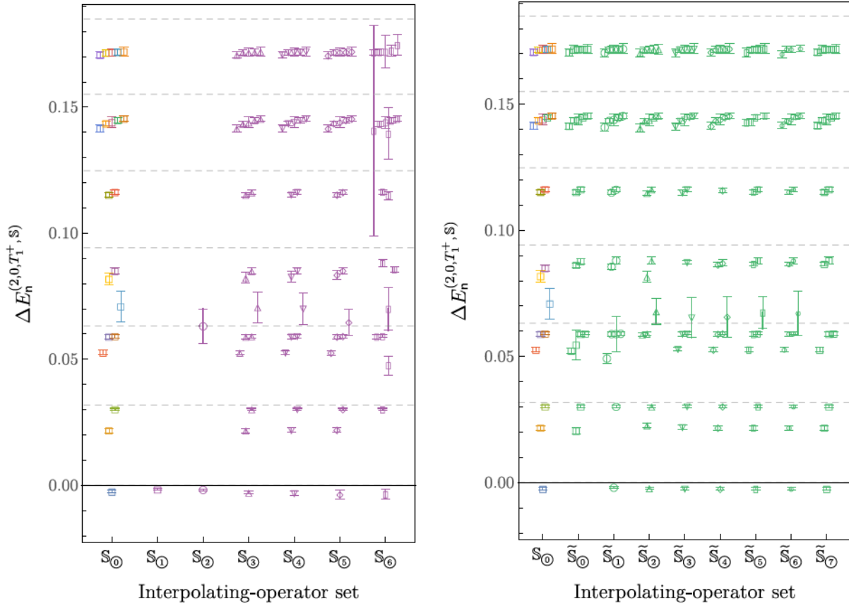
FIG. 26. FV energy shifts obtained using GEVP correlation functions with interpolating-operator set S_0^{(2,0,T_1^+)} (left column in each panel and corresponding to Figs. 19–21) are compared to results obtained using the interpolating-operator sets defined in Eq. (71) and featured in Fig. 25 (left) as well as the eight other interpolating-operator sets defined in Eq. (72) (right). The color coding for S_0^{(2,0,T_1^+)} energies follows that in Figs. 19–21, and the dashed lines show noninteracting two-nucleon energies as in Fig. 22.
