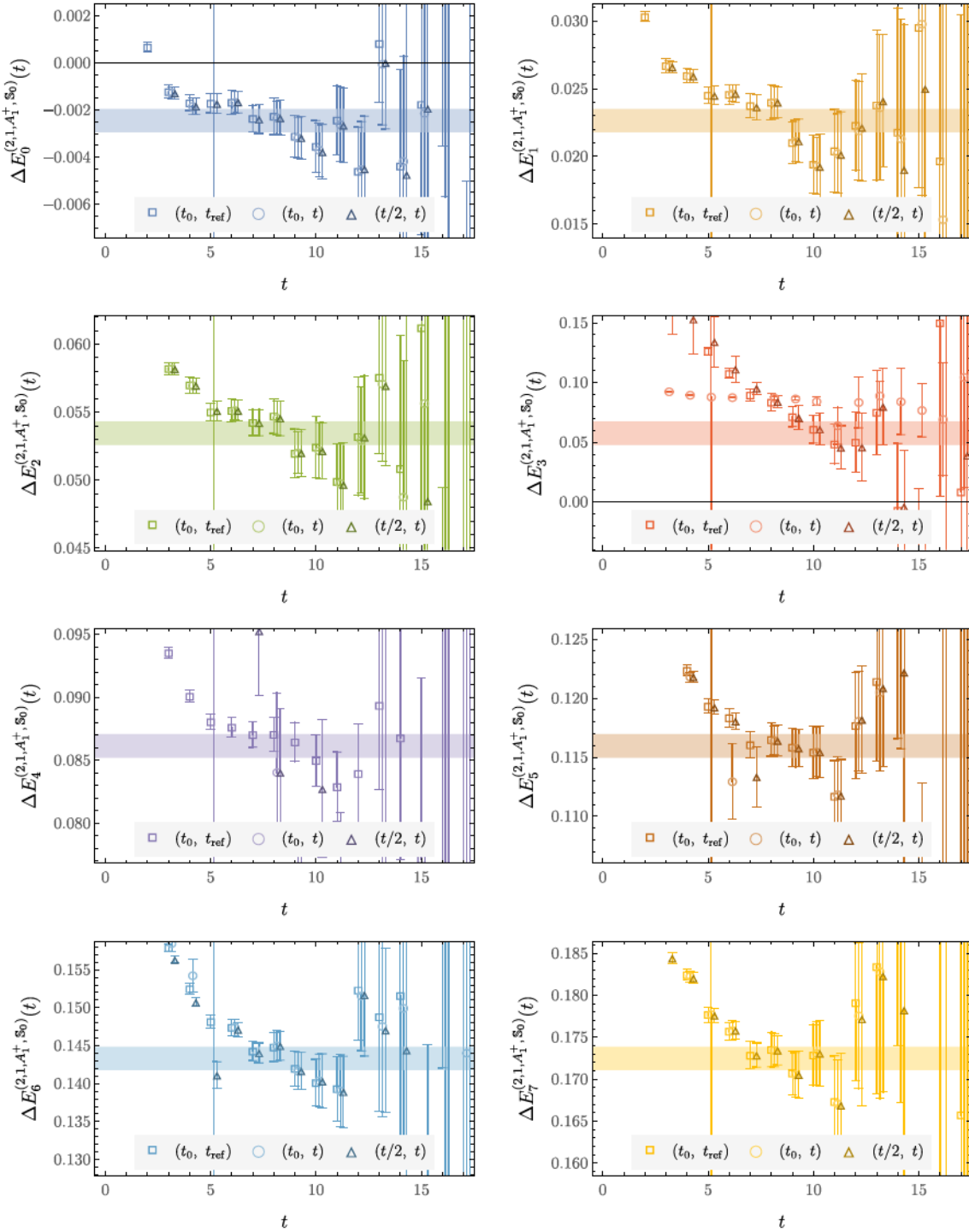
FIG. 41. The GEVP effective FV energy shifts determined using different schemes for choosing t_0 and t_{\text{ref}} to obtain GEVP eigenvectors using the interpolating-operator set S_0^{(2,1,A_1^+)} . Results with fixed t_0 = 5 and t_{\text{ref}} = 10 are identical to those in Fig. 7 and detailed in the main text, while the other results shown use fixed t_0 = 5 and variable t_{\text{ref}} = t and variable t_0 = t/2 and t_{\text{ref}} = t in analogy to Fig. 38.
