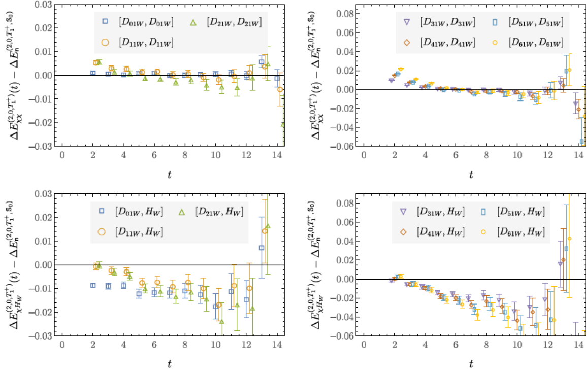
FIG. 27. The upper (lower) panels show differences between the effective FV energy shifts computed using correlation functions with dibaryon sources and sinks [D_{\mathfrak{s}1W}, D_{\mathfrak{s}1W}] (hexaquark sources and dibaryon sinks [D_{\mathfrak{s}1W}, H_W] ) and the fitted FV energy shifts for the \mathbb{S}_{\odot}^{(2,0,T_1^+)} GEVP energy levels that dominantly overlap with D_{\mathfrak{s}1W}^{(2,0,T_1^+)} , which are n \in \{0, 1, 3\} for the left panels and n \in \{7, 9, 11, 18\} for the right panels.
