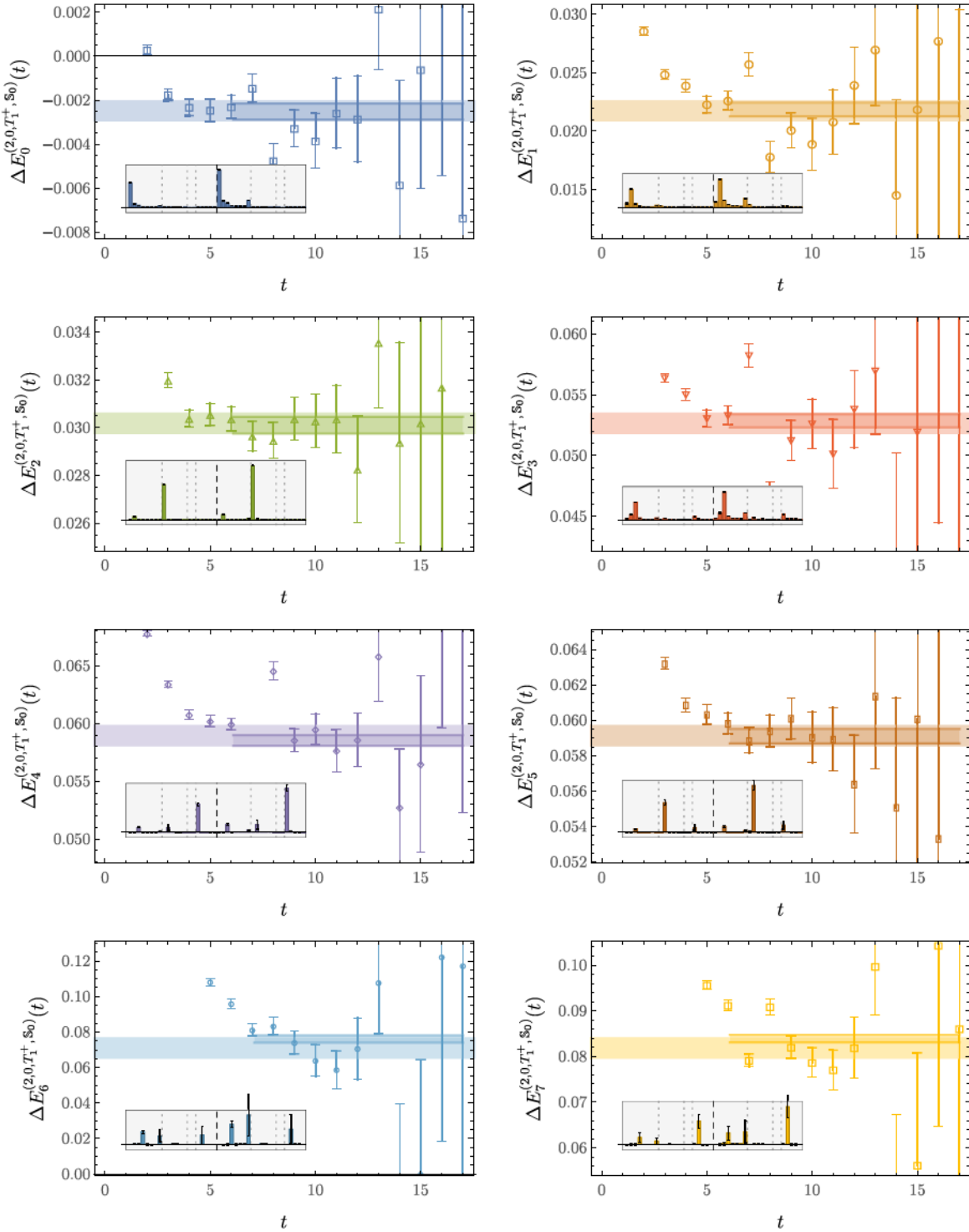
FIG. 19. Results for two-nucleon GEVP effective FV energy shifts for the lowest-energy GEVP correlation functions, n \in \{0, \dots, 7\} , with I = 0, \Gamma_J = T_1^+ obtained using the set S_{\otimes}^{(2,0,T_1^+)} . Statistical and systematic fit uncertainties are shown as in Fig. 7. Histograms of \mathcal{Z}_{n\chi}^{(2,0,T_1^+,S_0)} are analogous to the histograms in that figure and include a dashed line separating thin (left) and wide (right) quark-field smearing as well as dotted lines that further divide the operators into subsets corresponding to \Gamma_\ell = A_1^+, E^+, T_1^+, T_2^+ from left to right. Hexaquark operators appear rightmost among operators with \Gamma_\ell = A_1^+ .
