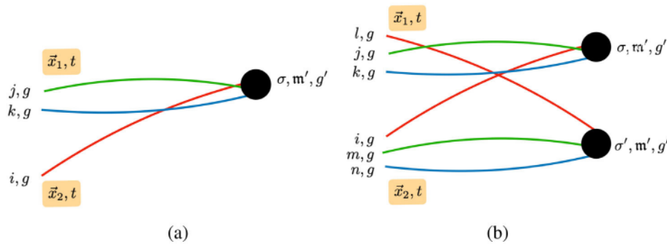
FIG. 4. Diagrams illustrating (a) the tensor structure of bilocal baryon blocks and (b) contributions to Eq. (36) involving them. Diagram (a) describes \mathcal{E}_{g \sigma m' g'}^{(q\pm)ijk}(\vec{x}_1, \vec{x}_2, t) with q = 1 , which includes a wave function e^{\pm i \vec{k}_{m'} \cdot \vec{y}} , weights w_{\alpha'}^{[N]\sigma} , and sums over spatial points \vec{y} \in \Lambda_S and weight index \alpha' collectively denoted by the black circle. Free indices \sigma , m' , and g' label the source baryon spin, wave function momentum, and quark-field smearing, respectively. Free spin-color indices i and j, k are associated with the sink positions \vec{x}_2 and \vec{x}_1 , respectively (other choices of q have different spin-color indices associated with \vec{x}_2 ), and g denotes the sink quark-field smearing. Diagram (b) similarly illustrates the product \mathcal{E}_{g \sigma m' g'}^{(1\pm)ijk}(\vec{x}_1, \vec{x}_2, t) \mathcal{E}_{g \sigma' m' g'}^{(1\mp)lmn}(\vec{x}_2, \vec{x}_1, t) appearing in Eq. (36).
