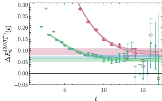
FIG. 24. The GEVP correlation functions for the n = 6 energy level dominantly overlapping with hexaquark operators, also shown in Fig. 19, is displayed offset in blue and compared with analogous GEVP correlation functions for interpolating-operator sets in which H_T^{(2,0,T_1^+)} is removed, in green, and with H_W^{(2,0,T_1^+)} removed, in purple.
