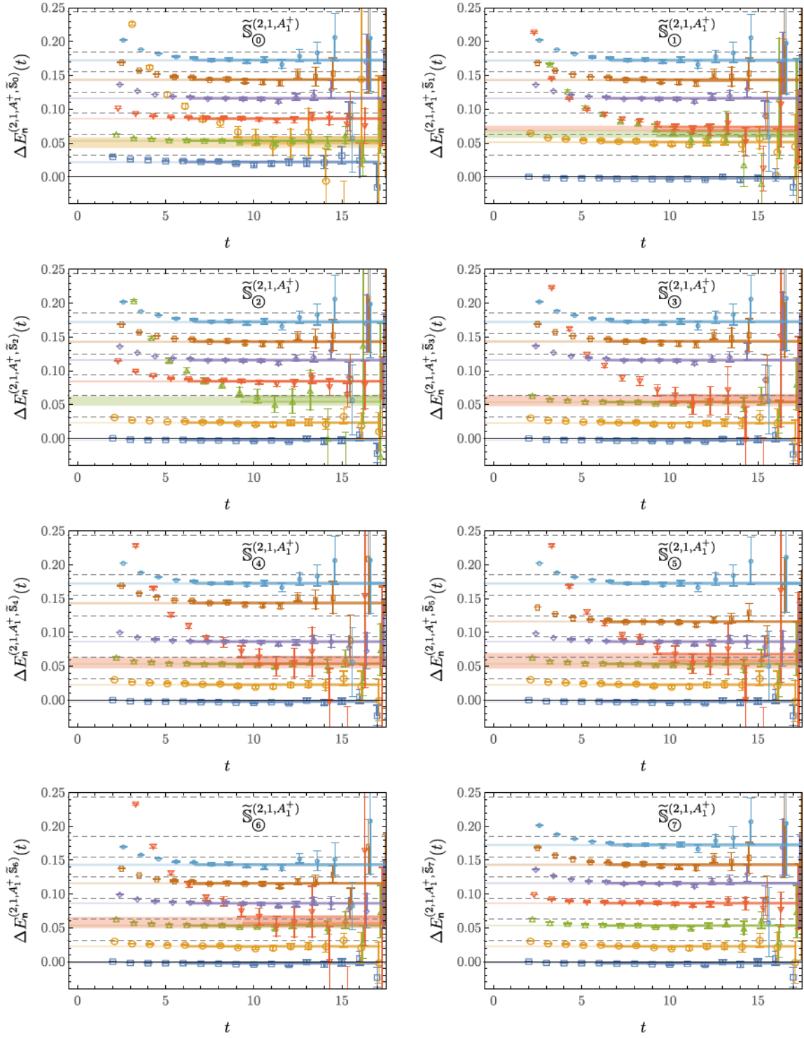
FIG. 43. The GEVP effective FV energy shifts analogous to Fig. 9 for interpolating-operator sets \tilde{S}_{\odot}^{(2,1,A_1^+)}, \dots, \tilde{S}_{\otimes}^{(2,1,A_1^+)} defined in Eq. (65).
