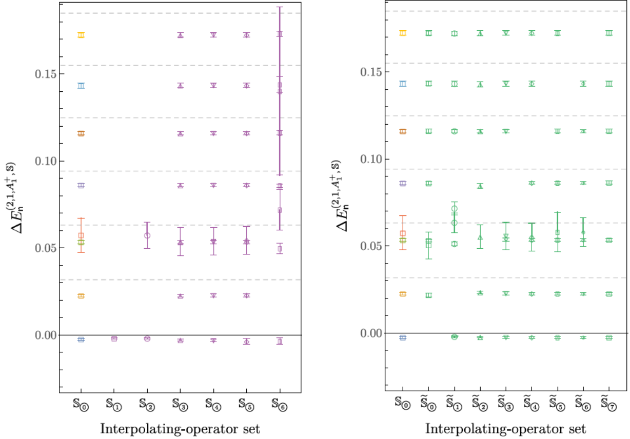
FIG. 12. FV energy shifts obtained using GEVP correlation functions with interpolating-operator set S_{\odot}^{(2,1,A_1^+)} (left column in each panel and corresponding to Fig. 7) are compared to results obtained using the interpolating-operator sets defined in Eq. (64) with ground-state energy shifts featured in Fig. 11 (left), as well as the eight other interpolating-operator sets defined in Eq. (65) (right). The color coding for S_{\odot}^{(2,1,A_1^+)} energies follows that in Fig. 7, and the dashed lines show noninteracting two-nucleon energies as in Fig. 9.
