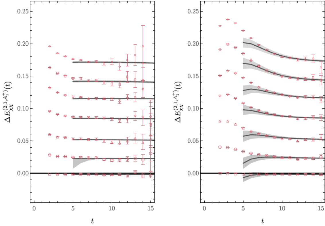
FIG. 15. Points with error bars show effective FV energy shifts for positive-definite dibaryon correlation functions [D_{s1g}, D_{s1g}] with s \in \{0, \dots, 6\} from bottom to top with wide (thin) quark-field smearing in the left (right) panel. Gray curves and bands show the central values and 68% confidence intervals for GEVP reconstructions that are obtained by inserting GEVP energy-level and overlap-factor results obtained using the interpolating-operator set \mathbb{S}_{\otimes}^{(2,1,A_1^+)} into the spectral representations for these correlation functions for all t \geq t_0 in analogy to Fig. 6. In particular, gray curves and bands are not obtained directly from fits to the correlation functions shown. Relatively large uncertainties on the higher-energy half of the spectrum lead to larger uncertainties in GEVP reconstructions at small t , particularly for the narrow smearing case in the right panel.
