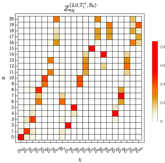
FIG. 23. Results for overlap factors \mathcal{Z}_{n_x}^{(2,0,T_1^+,S_0)} for the lower half of the GEVP energy eigenstates, which are shown as histograms in Figs. 19–21. Each column represents the sum of the overlap factors corresponding to the two quark-field smearings, \sum_g \mathcal{Z}_{nD_{\text{stg}}}^{(2,0,T_1^+,S_0)} or \sum_g \mathcal{Z}_{nH_g}^{(2,0,T_1^+,S_0)} , for each dibaryon or hexaquark operator. Uncertainties, shown by error bars in histograms in Figs. 19–21, are not shown here.
