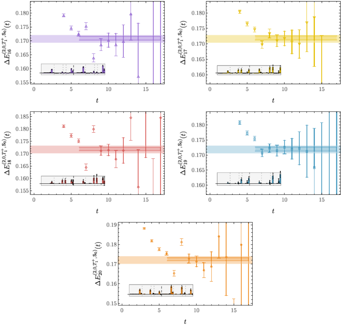
FIG. 21. Results for two-nucleon GEVP effective FV energy shifts for states n \in \{16, \dots, 20\} obtained using the interpolating-operator set \mathbb{S}_{\odot}^{(2,0,T_1^+)} . Symbols and bands are analogous to those in Fig. 19.
