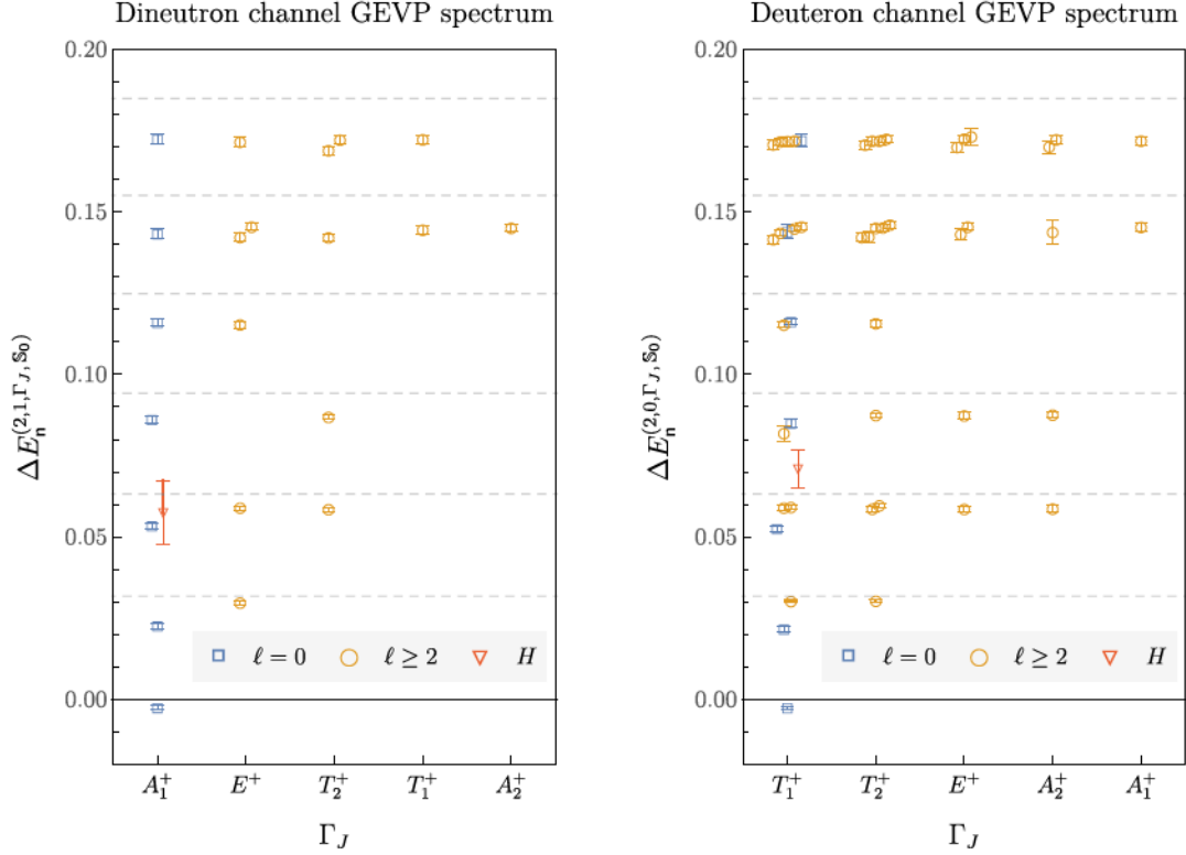
FIG. 33. GEVP energy levels below the single-nucleon first excited state with I = 1 ( I = 0 ) in the left (right) panel computed using interpolating-operator set S_{\otimes}^{(2,1,A_1^+)} ( S_{\otimes}^{(2,0,T_1^+)} ) for the \Gamma_J = A_1^+ ( \Gamma_J = T_1^+ ) irrep and using all available interpolating operators for the other irreps. Points with error bars show statistical and fitting systematic uncertainties added in quadrature and are distinguished by shape and color according to whether the interpolating operator with the largest overlap with each GEVP eigenstate is a dibaryon interpolating operator with \Gamma_\ell = A_1^+ associated with S -wave states in infinite volume, a dibaryon operator with \Gamma_\ell \neq A_1^+ associated with D -wave and higher partial-wave states, or a hexaquark operator. See Figs. 12 and 26 for summaries of the results, including quasilocal interpolating operators and other interpolating-operator sets. The horizontal lines indicate the positions of noninteracting two-nucleon energy levels.
