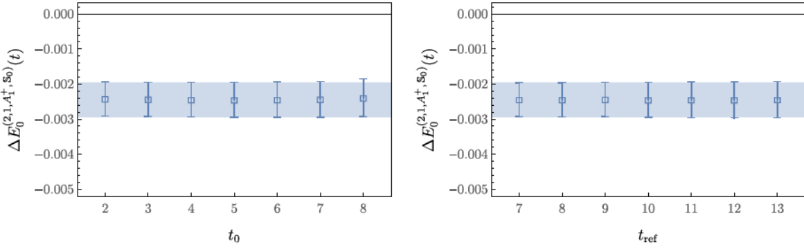
FIG. 39. Stability of I = 1, \Gamma_J = A_1^+ GEVP two-nucleon ground-state FV energy shifts using the interpolating-operator set \mathbb{S}_{\otimes}^{(2,1,A_1^+)} with respect to variation of t_0 and t_{\text{ref}} . Details are as in Fig. 37.
