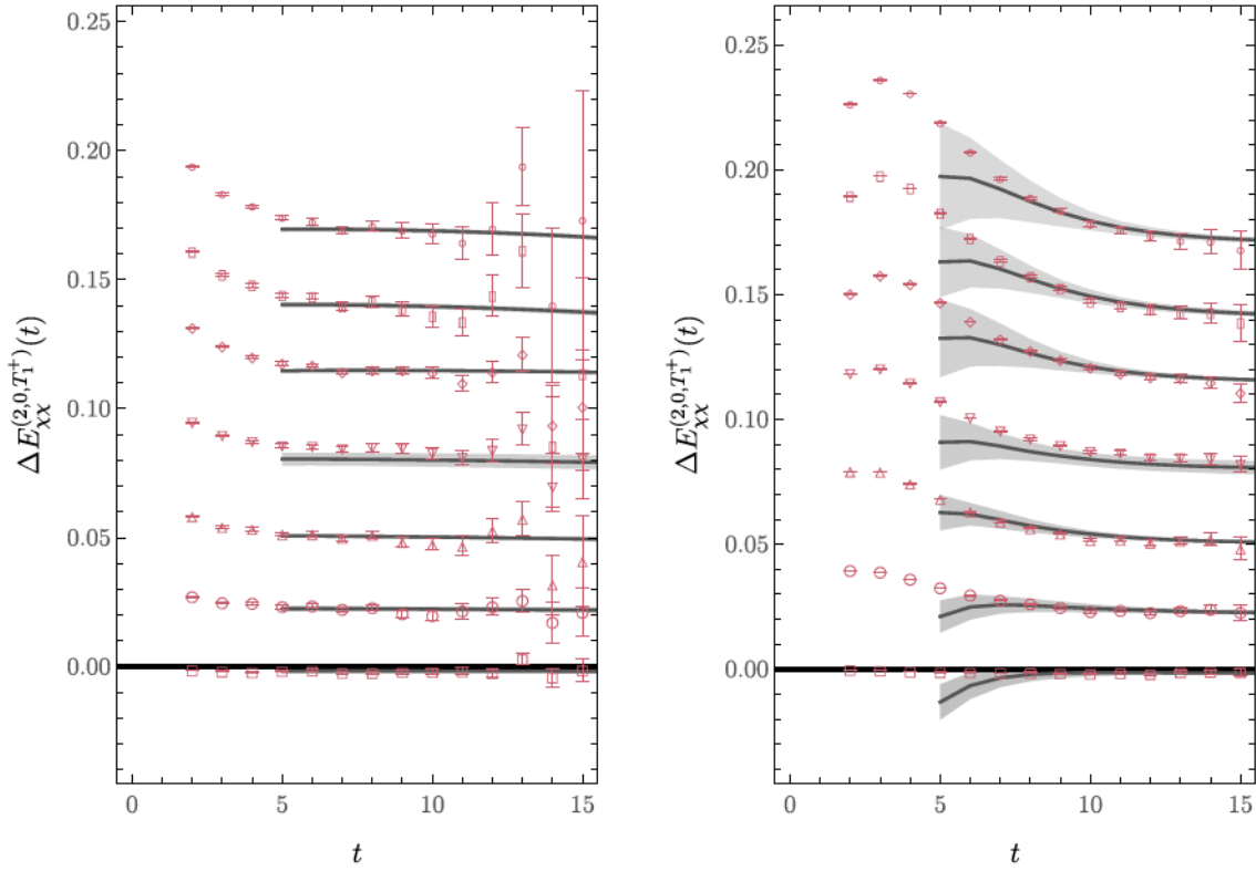
FIG. 29. GEVP reconstructions of [D_{s1g}, D_{s1g}] with s \in \{0, \dots, 6\} from bottom to top for wide (thin) quark-field smearing are shown in the left (right) panel. As in Fig. 15, gray curves and bands show the central values and uncertainties for GEVP reconstructions for t \geq t_0 . These are obtained by inserting GEVP energy level and overlap-factor results into spectral representations for the correlation functions and not from directly fitting the correlation functions shown.
