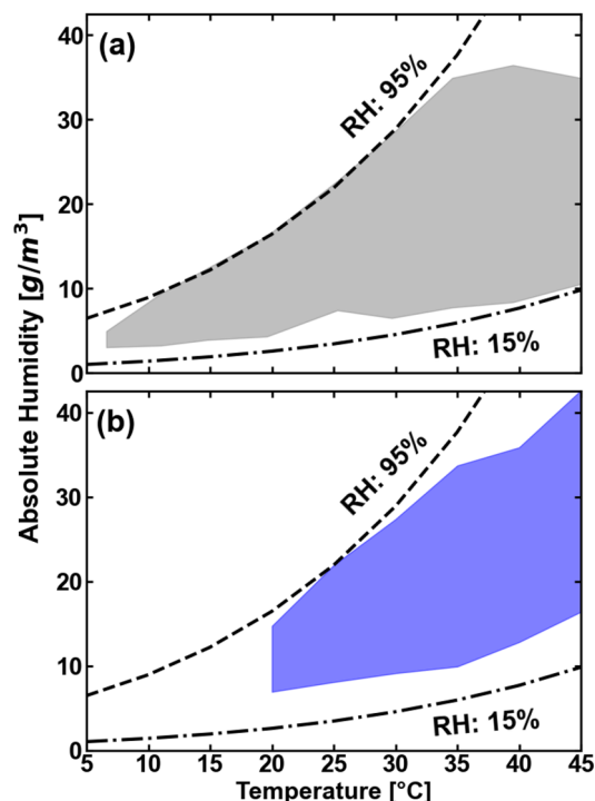
Figure 2. Temperature and absolute humidity regions covered in the study. (a) In the THz-TDS experiment, temperature change at \pm 5^{\circ}\text{C} steps over an interval of 6 ^{\circ}\text{C} to 45 ^{\circ}\text{C} . Absolute humidity values range from 2.7 to 36.9 \text{g/m}^3 . Each temperature value is fixed while the relative humidity change with step of \pm 5\% . For each TDS measurement, the climate chamber is stabilized at the corresponding humidity-temperature pair. (b) For the VNA experiment, the covered temperature interval ranges from 20 to 45 ^{\circ}\text{C} with \pm 5^{\circ}\text{C} steps. The absolute humidity values in this setup can be varied from 7.5 to 40.5 \text{g/m}^3 .
