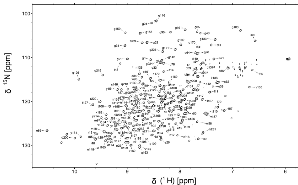
Fig. 1 ^{15}\text{N} - ^1\text{H} TROSY-HSQC NMR spectrum of mCherry with residue-specific assignments
