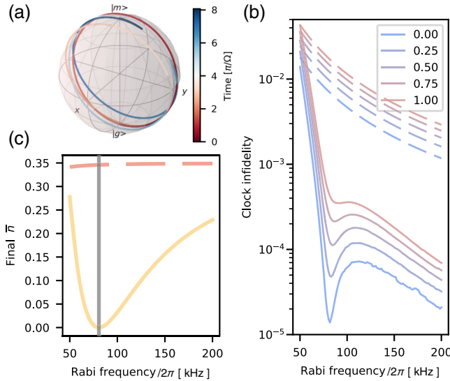
FIG. 10. Theoretical analysis of the MPP in a harmonic oscillator. The trap frequency is fixed to be 10 kHz. (a) Bloch sphere picture of the state evolution in a single MPP. (b) Theoretical state transfer infidelity after a single MPP for various initial average motional quanta, indicating a 2 orders-of-magnitude smaller infidelity, compared to a normal \pi pulse. The dashed line is for the normal \pi pulse, and the solid line is for the MPP. (c) Theoretical average motional state after a single MPP, assuming the initial state is in a motional ground state. A clear minimum can be observed at the Rabi frequency of approximately 80 kHz. We qualitatively confirm this feature is retained for another choice of initial temperature (not shown).
