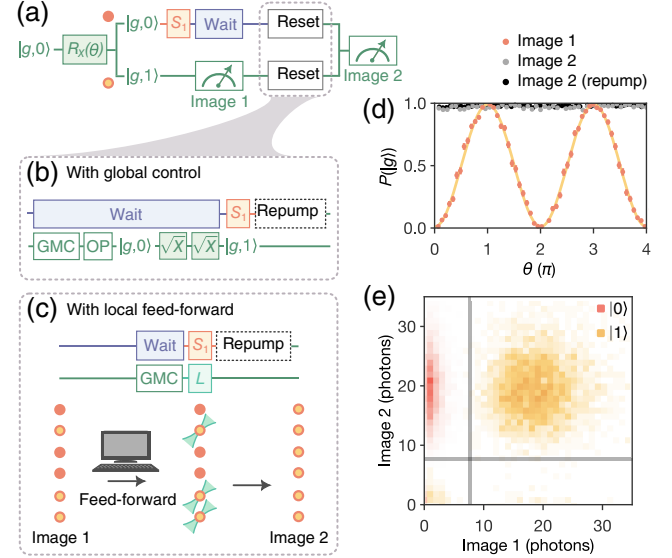
FIG. 4. Nondestructive state-sensitive detection. (a) Overview of the protocol. Note that S_1 turns spin |g,0\rangle dark, shelving it to the m manifold, while |g,1\rangle remains and appears bright for the image. The spins are then reset back to the g manifold. A final image checks for atom loss at the end of the procedure. (b,c) Two reset approaches employed. In panel (d), image 1 (yellow) is spin sensitive, resolving |0\rangle and |1\rangle populations of a |\psi\rangle = \cos(\theta/2)|0\rangle - i\sin(\theta/2)|1\rangle input state in g . Image 2 shows that the atoms can be reinitialized in g following spin detection via global control. No correction was applied to the data shown. The error bars indicate a 1\sigma confidence interval. (e) Two-dimensional histogram showing counts recorded in both images for atoms initially prepared in |0\rangle (orange) and |1\rangle (yellow) 2-ms wait time. Reinitialization in g , for this data set, was performed via a global control and repumping step before image 2.
