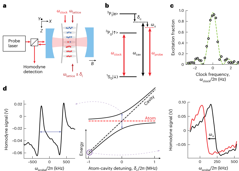
Fig. 1 | Optical clock with cQED architecture. a , ^{87}\text{Sr} atoms are trapped in a movable vertical optical lattice (by detuning one lattice beam by \delta_l ), enabling both independent squeezing and readout of two subensembles (red and blue) within the atomic cloud. The clock laser propagates along the vertical lattice, providing a global drive of the clock transition. Populations are measured non-destructively by means of homodyne detection of the laser probing the atom–cavity system. b , The relevant energy levels of ^{87}\text{Sr} . We prepare coherent superpositions between the clock states |\downarrow\rangle and |\uparrow\rangle . The frequency of the optical cavity \omega_{\text{cav}} is tuned near the |\downarrow\rangle \rightarrow |e\rangle transition to realize the atom–cavity
