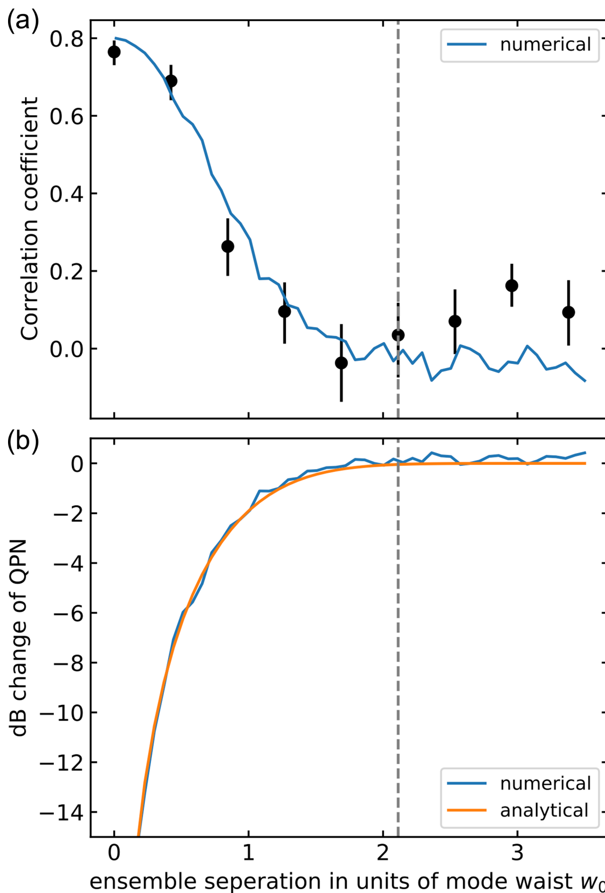
Extended Data Fig. 1 | Independence of atomic ensembles. a, Measured correlation coefficient between J_{z,A} and J_{z,B} versus the separation between the ensembles. (black circles). The blue line is a Monte Carlo simulation. b,
