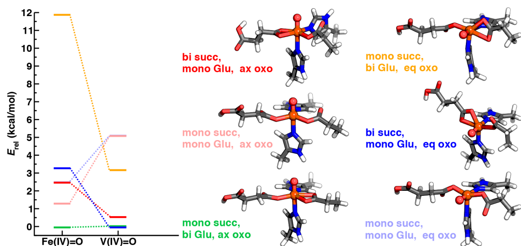
Figure 3. PBE0/def2-TZVP energies ( E_{\text{rel}} ) of isomers of M(IV)=O (M = Fe, V) intermediates shown relative to the most stable isomer for each intermediate in its ground spin state. Representative structures of Fe(IV)=O isomers are shown in the insets and labeled. (Top to bottom, left) Isomers are axial (ax) oxo, bidentate (bi) succinate (succ), monodentate (mono) Glu; axial oxo, monodentate succinate, monodentate Glu; axial oxo, monodentate succinate, bidentate Glu. (Top to bottom, right) Isomers are equatorial (eq) oxo, monodentate succinate, bidentate Glu; equatorial oxo, bidentate succinate, monodentate Glu; equatorial oxo, monodentate succinate, monodentate Glu. Hydrogen, carbon, nitrogen, oxygen, and iron are shown in white, gray, blue, red, and brown, respectively.
