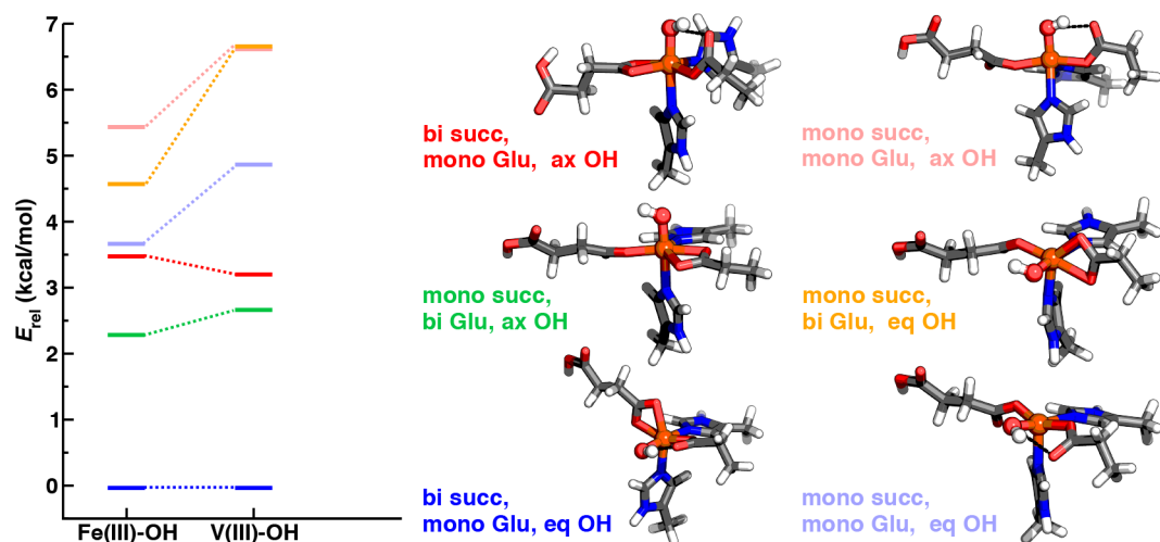
Figure 4. PBE0/def2-TZVP energies ( E_{\text{rel}} ) of isomers of M(III)–OH (M = Fe, V) intermediates shown relative to the most stable isomer for each intermediate in its ground spin state. Representative structures of Fe(III)–OH isomers are shown in the insets and labeled. (Top to bottom, left) Isomers are axial (ax) OH, bidentate (bi) succinate (succ), monodentate (mono) Glu; axial OH, monodentate succinate, bidentate Glu; equatorial (eq) OH, bidentate succinate, monodentate Glu. (Top to bottom, right) Isomers are axial OH, monodentate succinate,
