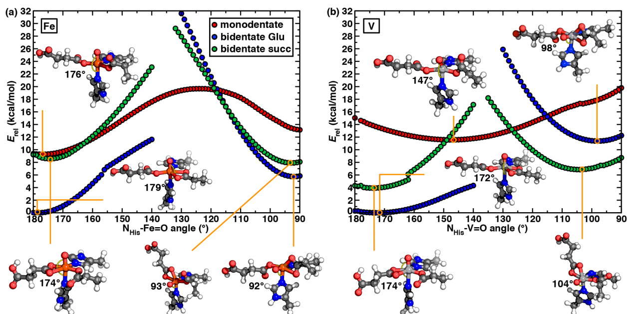
Figure 7. Reaction coordinates for isomerization between axial oxo and equatorial oxo with monodentate Glu and monodentate succinate (shown in red), bidentate Glu and monodentate succinate (shown in blue), and monodentate Glu and bidentate succinate (shown in green) for (a)
