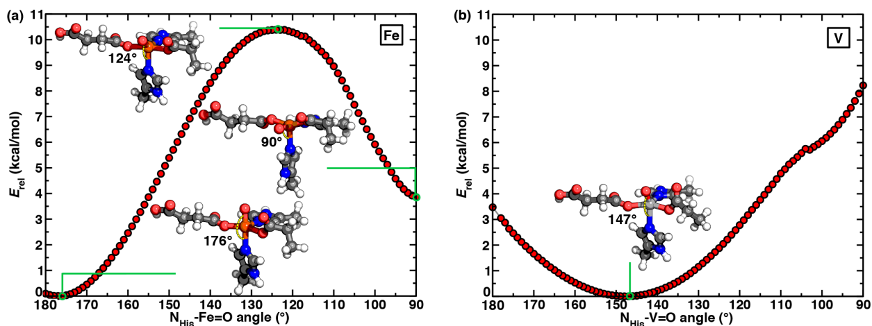
Figure 5. Reaction coordinates for isomerization between axial oxo and equatorial oxo with monodentate succinate and monodentate Glu for (a) Fe and (b) V active sites. The geometries corresponding to minima and transition states are shown as insets. The N_{\text{His}}\text{--M=O} angles (in ^\circ ,
