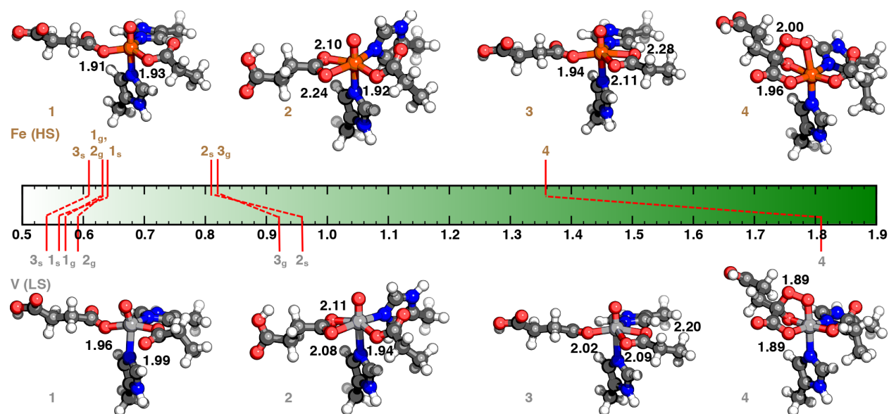
Figure 6. Scale demonstrating the Mayer bond orders of metal–Glu (g), metal–succinate (s), and metal– \alpha KG bonds of ground state high-spin (HS) Fe (top) and low-spin (LS) V (bottom) intermediates with monodentate Glu/succinate and bidentate Glu/succinate/ \alpha KG. The four intermediates shown are (1) M(IV)=O with monodentate succinate and monodentate Glu, (2) M(IV)=O with bidentate succinate and monodentate Glu, (3) M(IV)=O with monodentate
