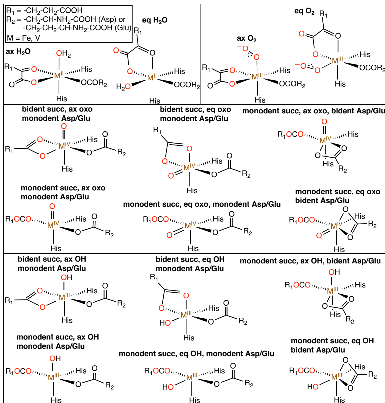
Figure 2. Isomers of four intermediates of non-heme hydroxylase active site formed during the catalytic cycle. M(II)-H_2O and M(III)-O_2 intermediates have two isomers: axial (ax) and equatorial (eq) H_2O/O_2 . M(IV)=O and M(III)-OH intermediates have six isomers: (i) bidentate (bident) succinate (succ), axial oxo/OH, monodentate (monodent) Asp/Glu (ii) bidentate succinate, equatorial oxo/OH, monodentate Asp/Glu (iii) monodentate succinate, axial oxo/OH, bidentate Asp/Glu (iv) monodentate succinate, equatorial oxo/OH, bidentate Asp/Glu (v) monodentate succinate, axial oxo/OH, monodentate Asp/Glu (vi) monodentate succinate, equatorial oxo/OH, monodentate Asp/Glu. The metal, M=Fe, V , is shown in brown, and the oxidation state for each intermediate is specified.
