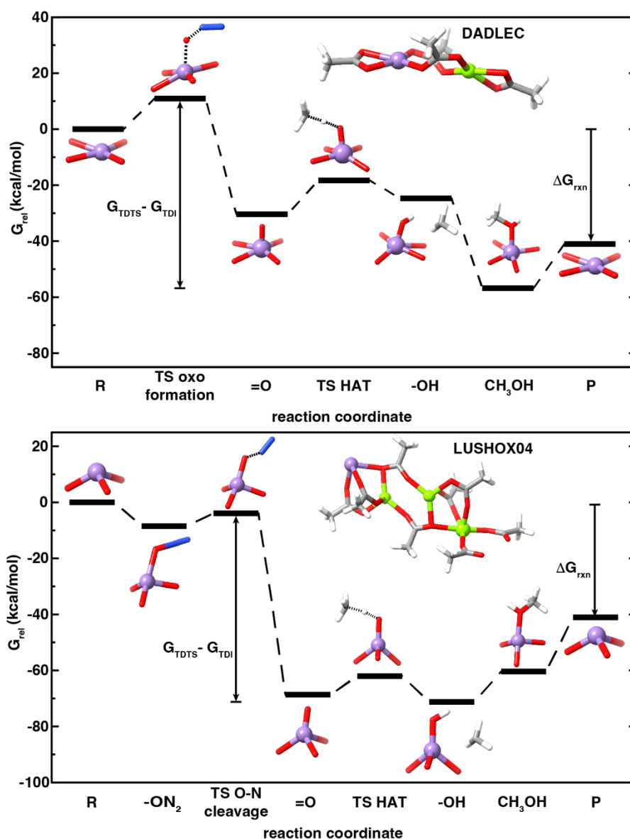
Figure 7. Gibbs free energy landscapes of (top) Mn(HTPA)(DMF) 2 n ·H 2 O (CSD refcode DADLEC) and (bottom) [Mn 2 (BDC) 2 (DMF) 2 ] n (CSD refcode LUSHOX04) with SBU and active site structures shown as insets. We draw the reaction coordinate from the reactants (R) (plus CH 4 , and N 2 O). DADLEC proceeds directly through an oxo formation TS (TS oxo formation) to form the metal-oxo intermediate (=O) while LUSHOX04 first forms a complex with N 2 O (-ON 2 ),
