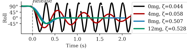
Fig. 7. Counterweight vs 1D Damping: Final Template flybar roll angle response with different counterweights show increased damping with increased counterweight. MoCap cameras occasionally miss data points.
