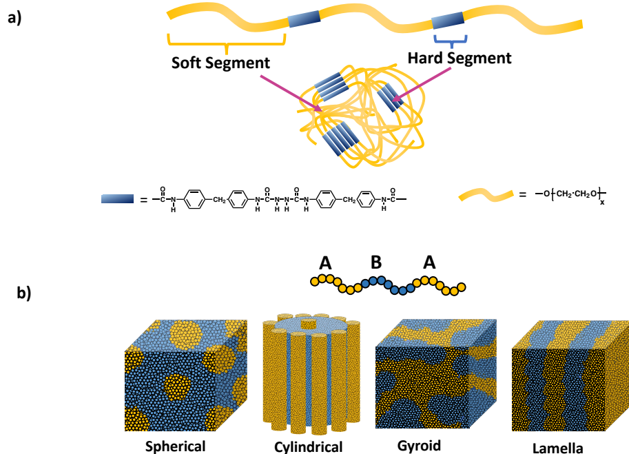
Scheme 12 :a) polyurethane networks and b) self-assembly of ABA triblock copolymers into different domains (spherical, cylindrical, gyroid, and lamella) through physical crosslinks.
