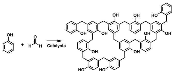
Scheme 1: Synthesis of Bakelite by condensation of phenol and formaldehyde. 6
