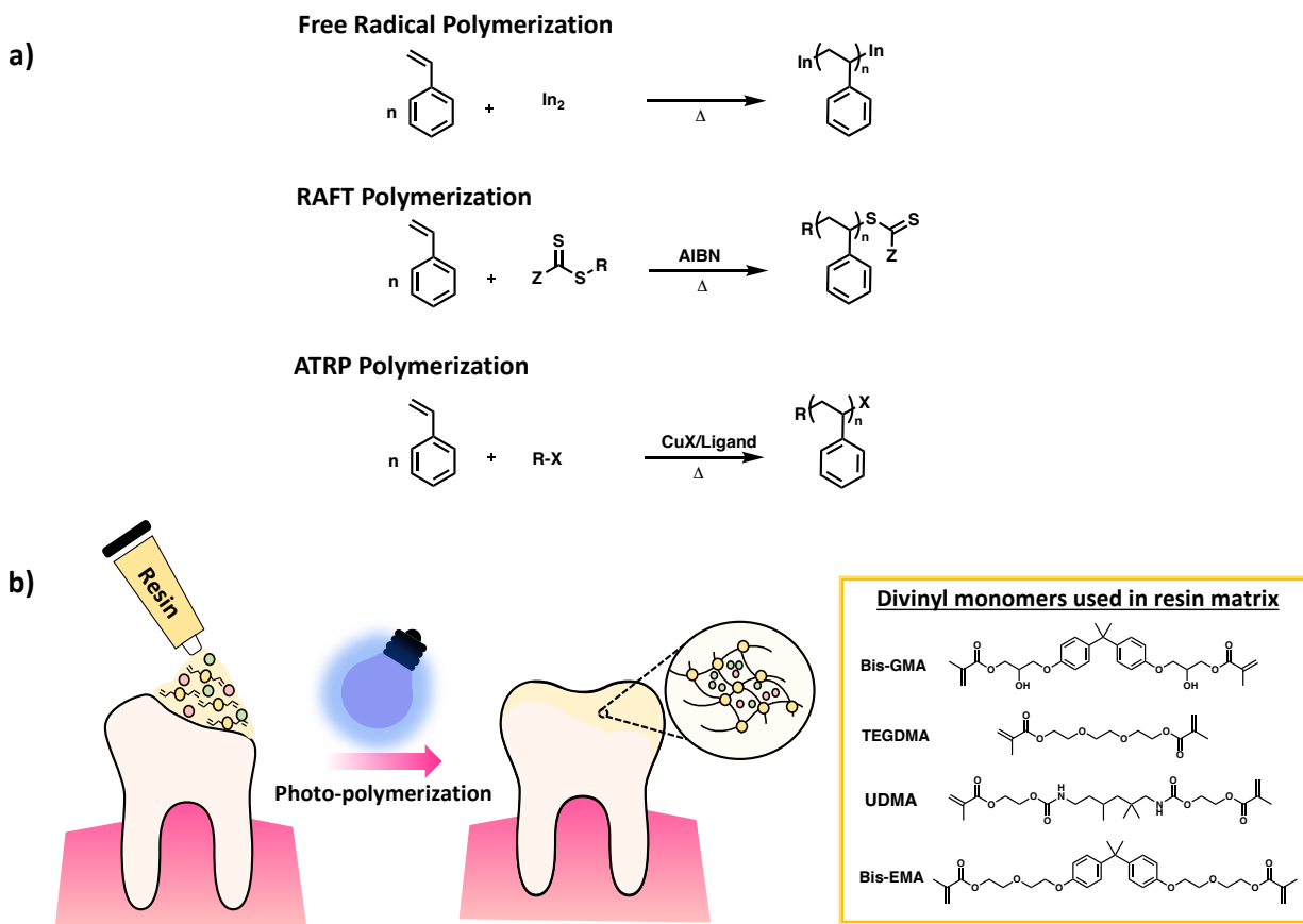
Scheme 8: Schematic diagram of a) synthesis of poly(styrene) via FRP, RAFT and ATRP. b) Crosslinking of DVMs for dental resins 50
