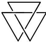
Figure 1. Trefoil knot.
