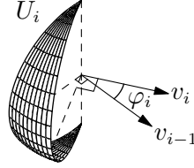
Figure 3. Spherical slice.
