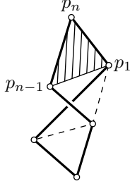
Figure 2. Triangular isotopy.
