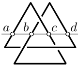
Figure 7. Alternated quadrisecant.
