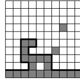
Figure 9. Colored set.
