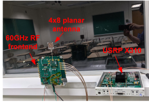
Fig. 3: Experimental setup in a classroom. Fig. 4: A picture of mmWave AP.
