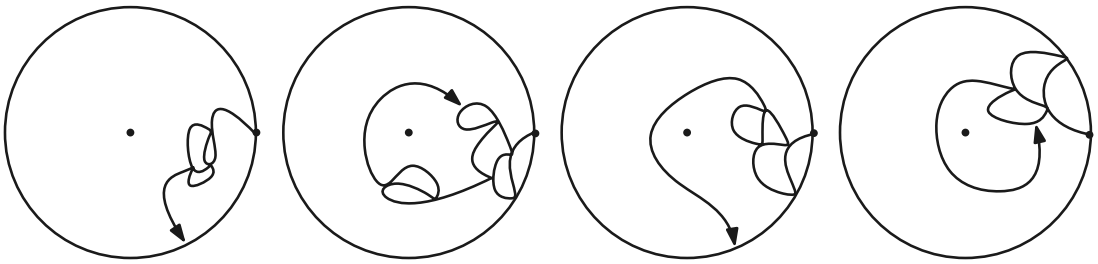
FIGURE 3 From left to right, the process \theta_0^\varepsilon does the following at the illustrated time: hits 0, hits 0, hits neither 0 nor 2\pi , hits 2\pi . The rightmost image is, therefore, an illustration of the time \tau_0^\varepsilon .
