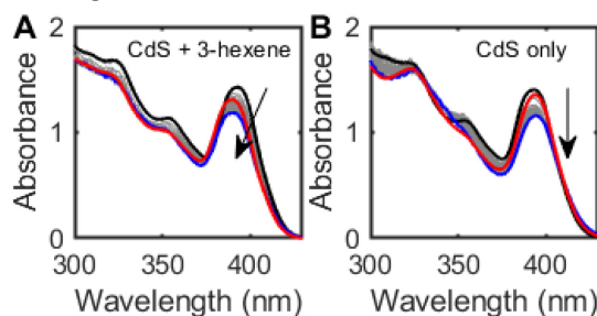
Figure 2. (A) Absorption spectra of a hexanes suspension of OA-capped CdS QDs ( d \sim 2.7 nm, 6.9 \mu\text{M} ) and cis -3-hexene (80 equiv/QD) before (black) and after (blue) irradiation under \text{N}_2 atmosphere ( \lambda = 370 nm, 24 h). The red trace shows the absorption spectrum of the sample after opening to air. (B) Absorption spectra of a hexanes suspension of CdS QDs under similar conditions, without added cis -3-hexene.
