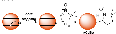
Scheme 2. Proposed radical addition pathway of a photogenerated surface-trapped hole to DMPO to form 2 CdSe .
