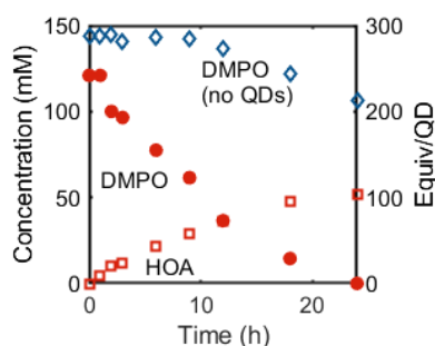
Figure 6. Concentrations of DMPO (red circles) and oleic acid (red squares) in a \text{C}_6\text{D}_6 mixture of OA-capped CdSe QDs ( d \sim 3.6 nm, 0.5 mM) and DMPO (300 equiv/QD) over time during irradiation ( \lambda = 440 nm, 200 \text{mW}/\text{cm}^2 ). The concentration of a \text{C}_6\text{D}_6 solution of DMPO during irradiation ( \lambda = 370 nm, 100 \text{mW}/\text{cm}^2 ) in the absence of QDs is included for comparison (blue diamonds).
