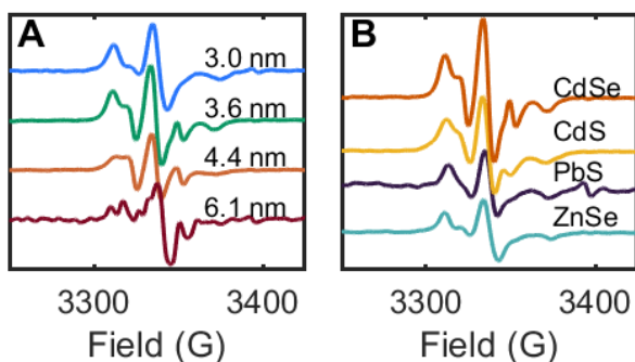
Figure 8. (A) Room temperature X-band EPR spectra of toluene suspensions of CdSe QDs of different sizes after thermal treatment with DMPO (1000 equiv/QD) and GPC purification. (B) Room temperature X-band EPR spectra of toluene suspensions of different QD materials after thermal treatment with DMPO and GPC purification.
