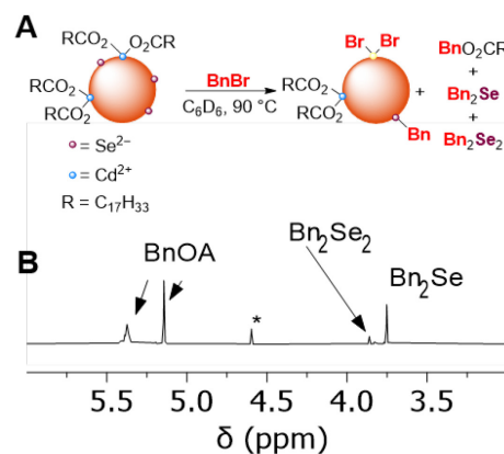
Figure 7. (A) Scheme showing that benzylation of carboxylate ligands and of surface selenide ions of CdSe QDs upon treatment with benzyl bromide. (B) Truncated ^1\text{H} NMR spectrum showing benzylic resonances of a \text{CDCl}_3 solution of molecular products formed upon heating a benzene mixture of OA-capped CdSe QDs ( d \sim 3.6 nm, 0.5 mM) and BnBr (50 equiv/QD) at 90 °C for 15 h. (*) indicates a \text{Bn}_2\text{O} impurity.
