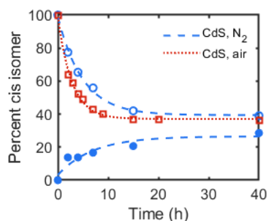
Figure 1. Cis-trans isomerization of 3-hexene in C_6D_6 with OA-capped CdS QDs ( d \sim 2.7 nm, 1 mol %) during irradiation ( \lambda = 370 nm, 100 mW/cm 2 ) plotted as percentage cis isomer over time. Open markers plot values starting from 100% trans -3-hexene at t = 0 ,
