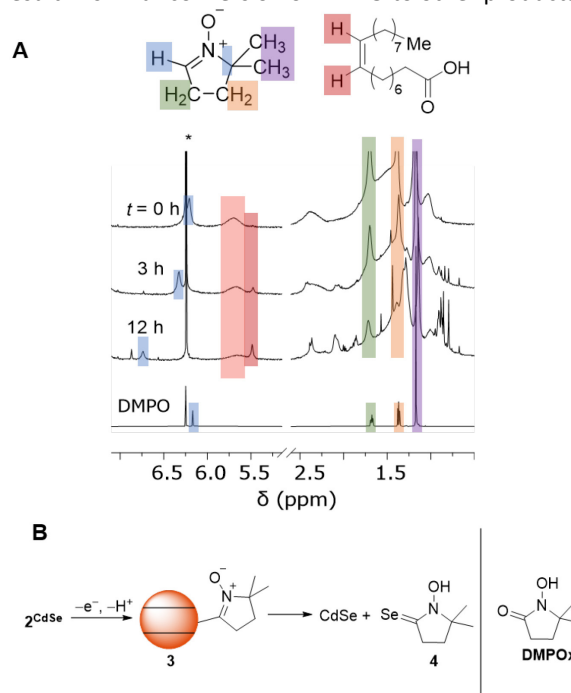
Figure 5. (A) 1 H NMR spectra of a C 6 D 6 mixture of zinc blende OA-capped CdSe QDs ( d \sim 3.6 nm) and DMPO (300 equiv/QD) during irradiation ( \lambda = 440 nm, 200 mW/cm 2 ). (B) Proposed oxidative formation of DMPO-derived diamagnetic products from 2 CdSe .
