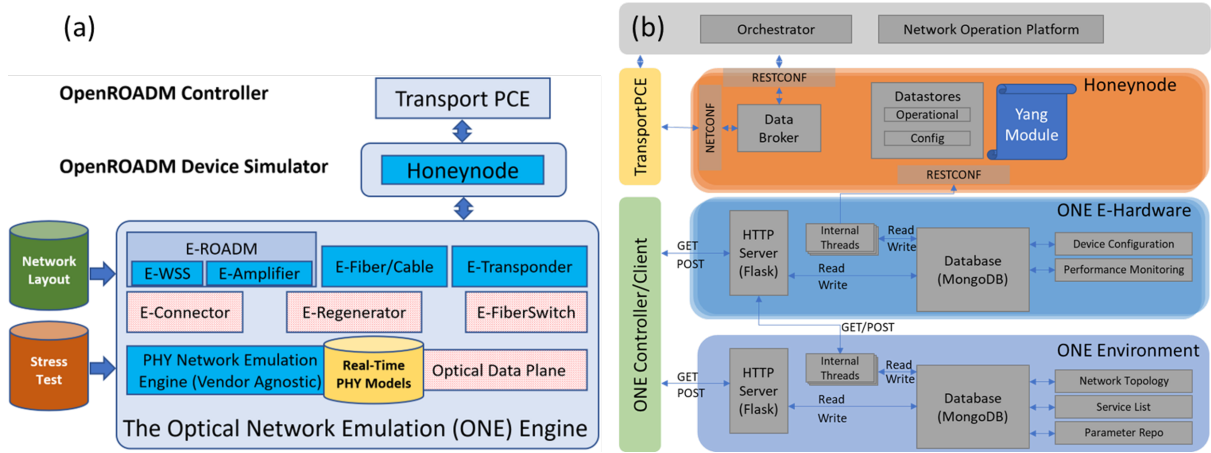
Fig. 1. (a) ONE decentralized architecture and key modules – dashed red modules not yet available and (b) OpenROADM network emulation through Honeynode and ONE engine
