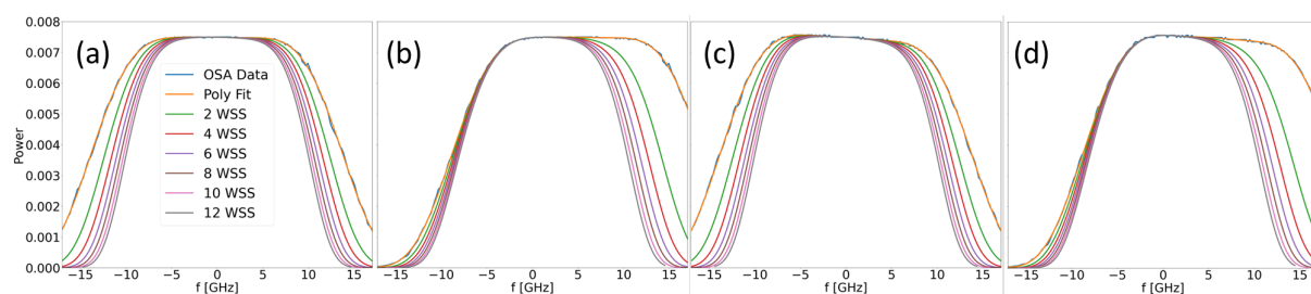
Fig. 2. (a,c): Normalized signal power spectra using polynomial terms for two launched power levels as they cross increasing number of WSS devices; (b,d): Signal central frequency offset is 5 GHz
