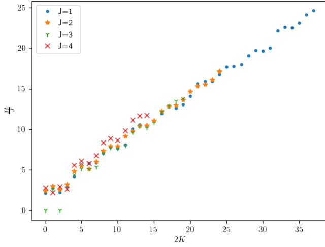
FIG. 5. For each J we plot the largest mass scaled by J as a function of 2K .
