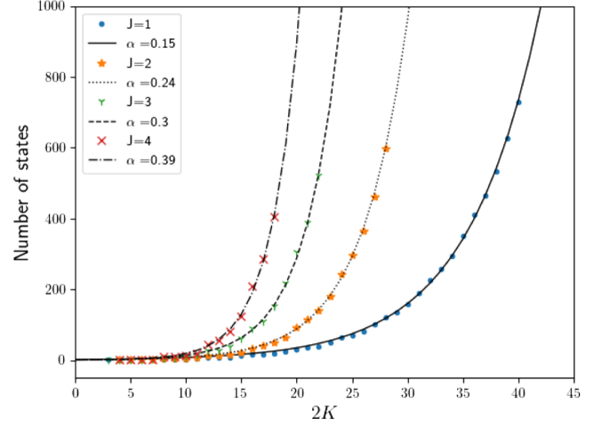
FIG. 6. We have plotted the number of states as a function of 2K for J = 1, 2, 3, 4 . We fitted each curve to Ce^{2\alpha K} and list the \alpha values for each curve.
