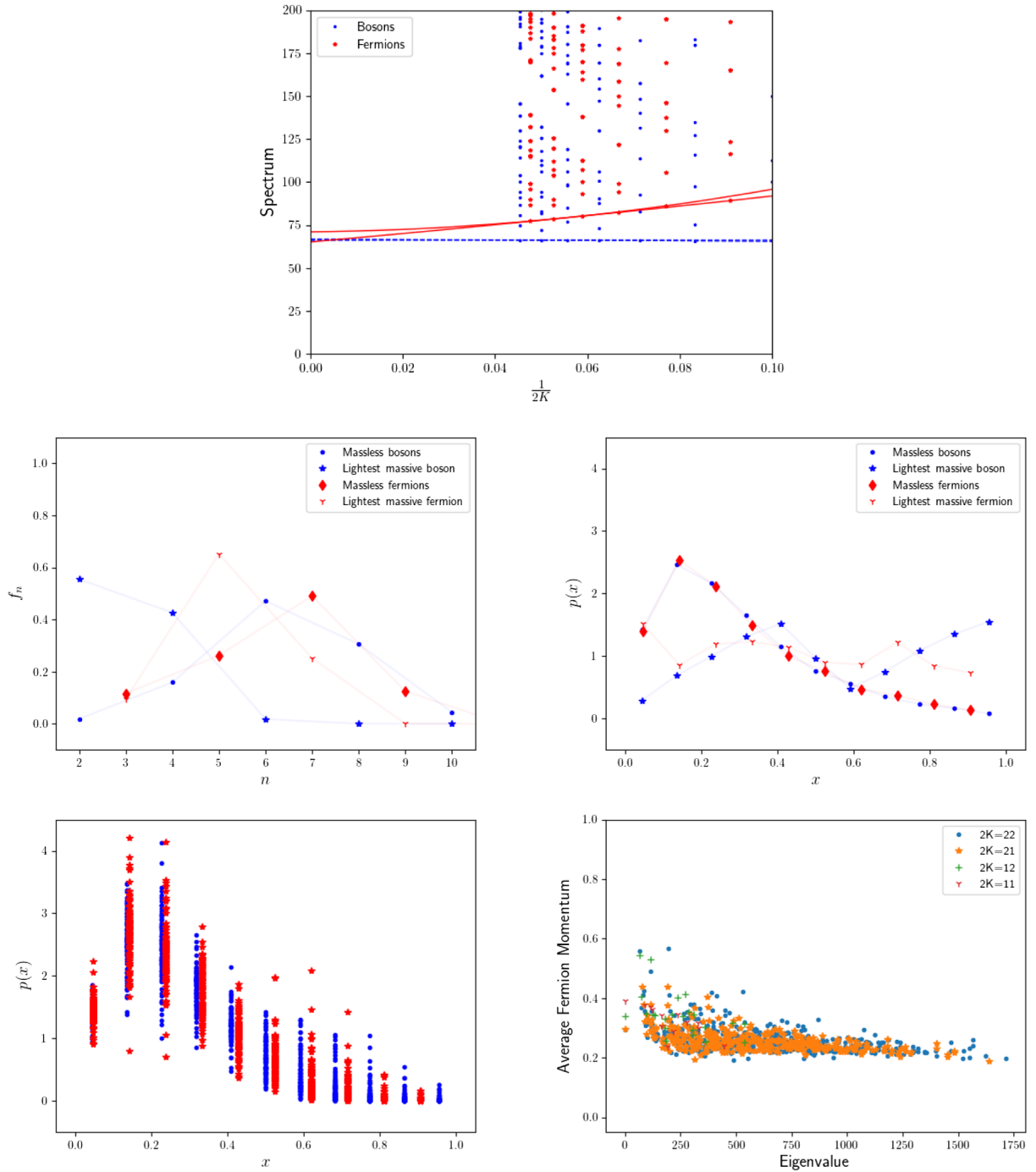
FIG. 3. Analysis of J = 3 . The color red is reserved for fermionic states and the color blue for bosonic states. The extrapolated lowest nonzero masses in the top panel are listed in Table I.
