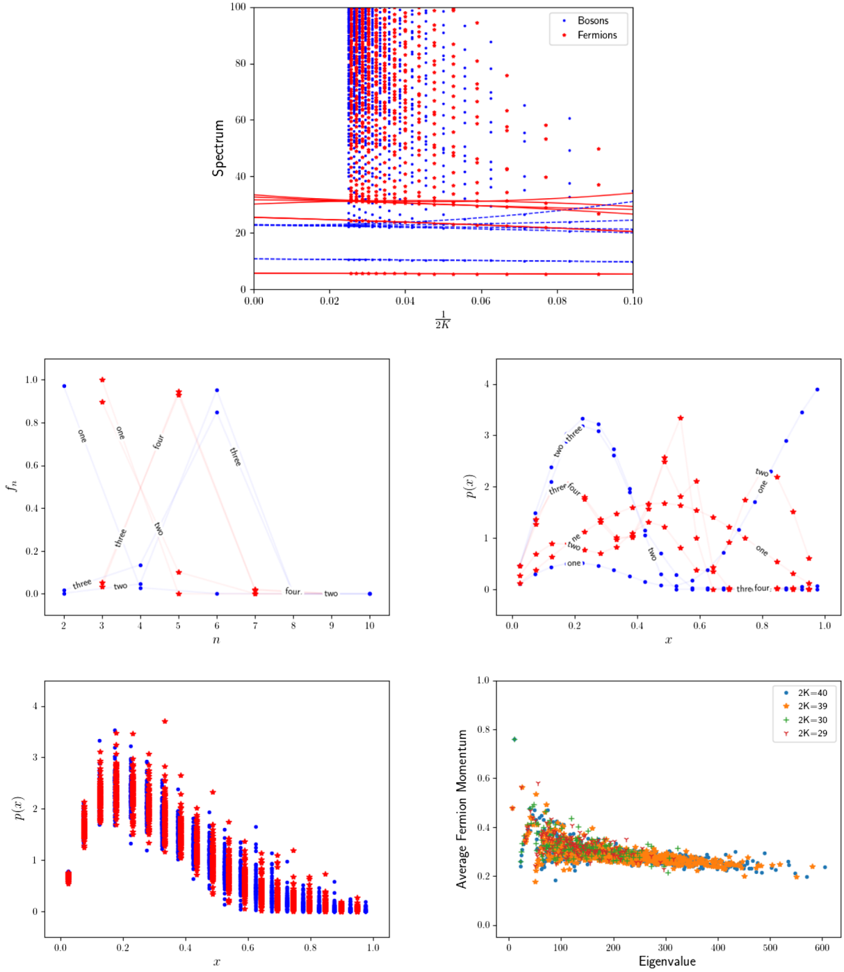
FIG. 1. Analysis of J = \frac{1}{2} . The color red is reserved for fermionic states and the color blue for bosonic states. The extrapolated masses in the top panel are listed in Table I.
