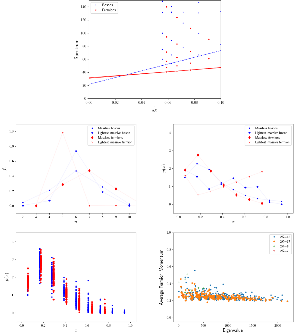
FIG. 4. Analysis of J = 4 . The color red is reserved for fermionic states and the color blue for bosonic states. The extrapolated lowest nonzero masses in the top panel are listed in Table I.
