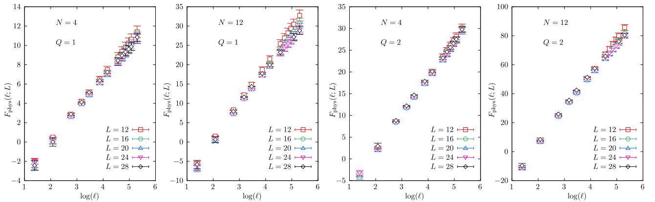
FIG. 4. The free energy F_{\text{phys}}(\ell, L) converted to physical units is shown as a function of \ell . The data points at fixed L are shown using the different colored symbols. The values of (Q, N) in the panels from left to right correspond to (1, 4) , (1, 12) , (2, 4) , (2, 12) , respectively.
