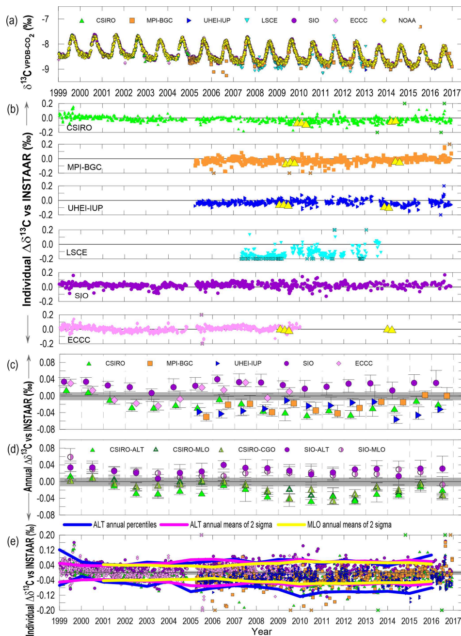
Figure 2. Atmospheric \delta^{13}\text{C} – \text{CO}_2 comparison results, in per mill (‰), from flask samples taken at ALT, MLO, and CGO by seven laboratories. (a) Time series of each laboratory's measurements at ALT, showing long-term trends and seasonal patterns in the records. (b) Individual ALT \delta^{13}\text{C} – \text{CO}_2 differences (laboratory minus INSTAAR) (in ‰). Differences exceeding the y-axis range are plotted with an “X” symbol on the outer axis. Results from the WMO/IAEA Round Robin experiments are overlaid in yellow triangles. The shaded grey band around the zero line indicates the WMO-GAW-recommended measurement agreement goal of \pm 0.01 ‰. (c) Annual median \delta^{13}\text{C} – \text{CO}_2 differences (laboratory minus INSTAAR) at ALT (in ‰), with the lower and upper limits of estimated 95 % CI. (d) Annual median \delta^{13}\text{C} – \text{CO}_2 differences and 95 % CI (in ‰), of CSIRO minus INSTAAR at MLO and CGO, and SIO minus INSTAAR at MLO. Also included are results from ALT. (e) Individual measurement differences (laboratory minus INSTAAR) at ALT (in ‰) for all the laboratories as a collective. Some extreme outliers have been removed to produce the results. The annual 2.5th and 97.5th percentiles of the entire difference distribution from all laboratories at ALT are shown in blue ( -0.09 ‰ to +0.07 ‰). The pink lines show the annual means of \pm 2\sigma variations of weekly sampling episodes at ALT ( \pm 0.06 ‰), and the yellow lines show the annual means of \pm 2\sigma variations of weekly sampling episodes at MLO ( \pm 0.05 ‰).
