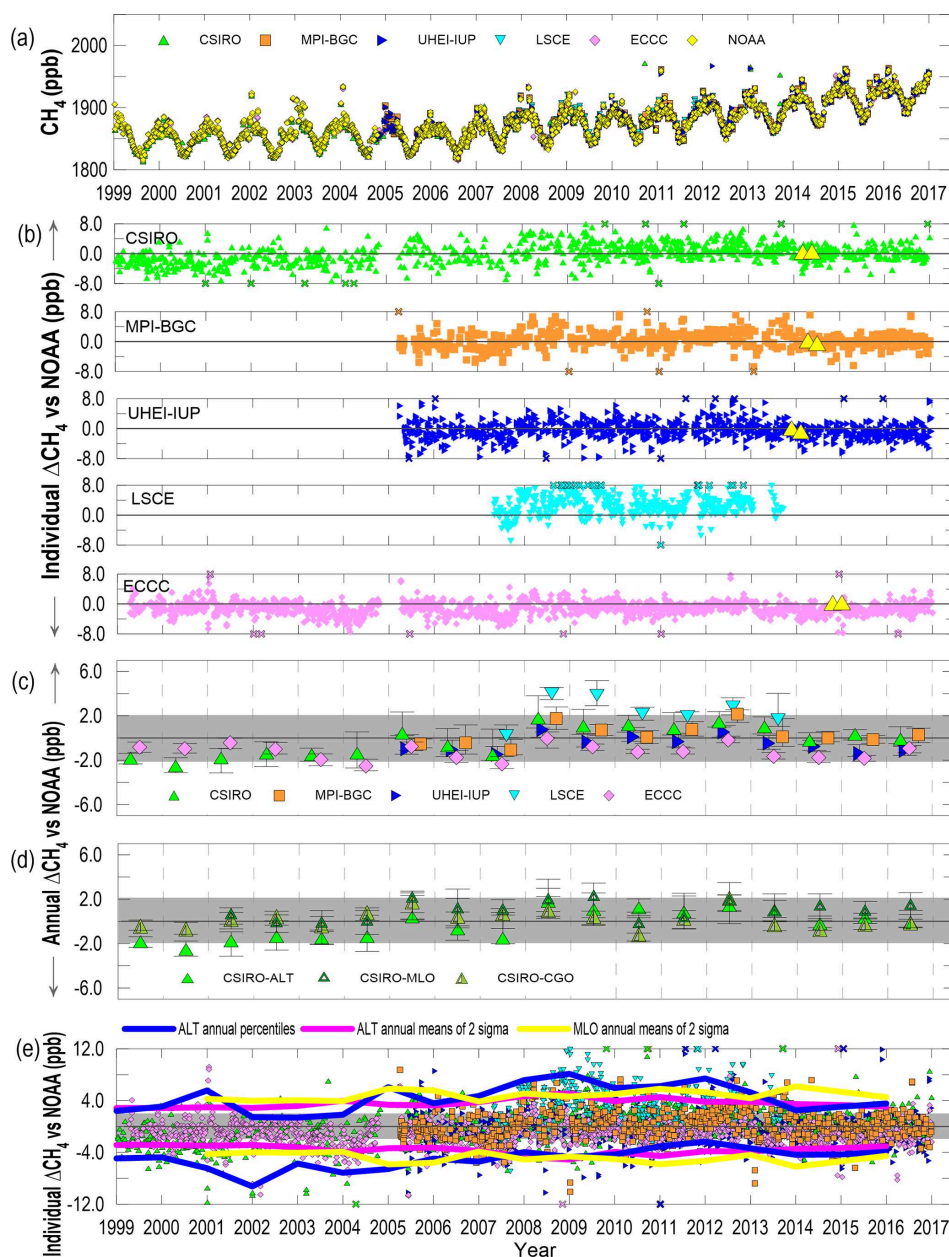
Figure 4. Atmospheric CH 4 comparison results (in ppb) from flask samples taken at ALT, MLO, and CGO by six laboratories (CSIRO, MPI-BGC, UHEI-IUP, LSCE, ECCC, and NOAA). (a) Time series of each laboratory's measurements at ALT, showing long-term trends and seasonal patterns in the records. (b) Individual CH 4 differences (laboratory minus NOAA) at ALT (in ppb). Differences exceeding the y-axis range are plotted with an "X" symbol on the outer axis. Results from the WMO/IAEA Round Robin experiments are overlaid in yellow triangles. The shaded grey band around the zero line indicates the WMO-GAW-recommended measurement agreement goal of \pm 2.0 ppb. (c) Annual median CH 4 differences (laboratory minus NOAA) at ALT (in ppb) with the lower and upper limits of estimated 95 % CI. (d) Annual median CH 4 differences and 95 % CI (in ppb) of CSIRO minus NOAA at MLO and CGO. Also included are results from ALT. (e) Individual differences (laboratory minus NOAA) at ALT (in ppb) for all the laboratories as a collective. Some extreme outliers have been removed to produce the results. The annual 2.5th and 97.5th percentiles of the entire difference distribution from all laboratories at ALT are shown in blue ( -4.86 to +6.16 ppb). The pink lines show the annual means of \pm 2\sigma variations of weekly sampling episodes at ALT ( \pm 3.62 ppb), and the yellow lines show the annual means of \pm 2\sigma variations of weekly sampling episodes at MLO ( \pm 4.88 ppb).
