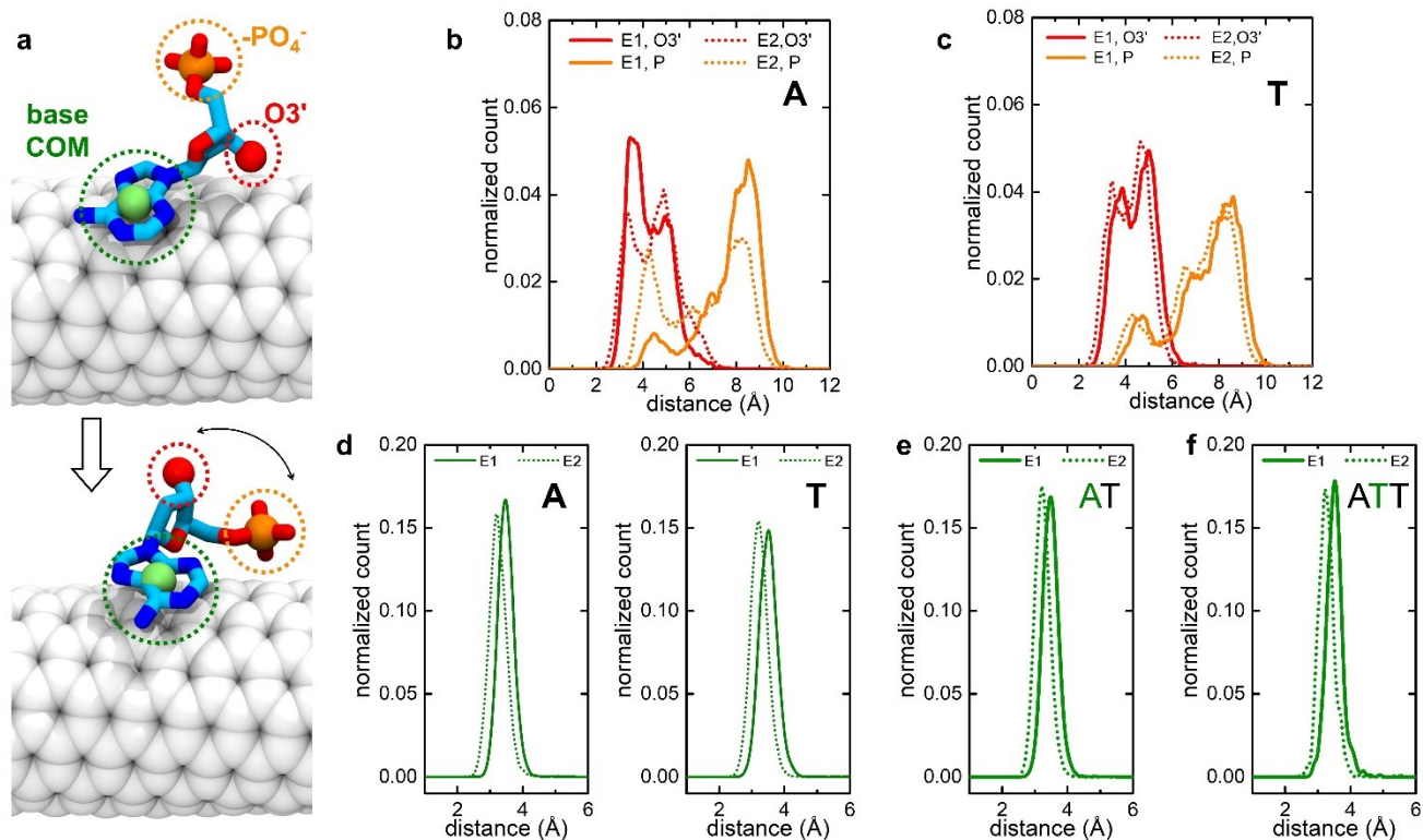
Figure 1. Binding modes and distances between nucleotides and surfaces of SWNT enantiomers. a) Snapshots of two representative binding modes for A nucleotide at the (7,5) SWNT surface. SWNT atoms are shown as white spheres, and DNA heavy atoms are colored in light blue (C), dark blue (N), red (O) and orange (P). Hydrogen atoms are not shown for clarity. The center of mass of the base is shown as a green sphere. The M and P enantiomers of the SWNT with chiral index (7,5) are referred to as E1 and E2, respectively, throughout the paper. b) Distribution of distances between phosphate groups or O3' atoms and SWNT surfaces, determined for A nucleotide binding to two enantiomers of (7,5) SWNT. c) Distribution of distances between phosphate groups or O3' atoms and SWNT surfaces, determined for T nucleotide binding to two enantiomers of (7,5) SWNT. d) Distribution of distances between base centers of mass and SWNT surfaces, determined for single A and T nucleotides binding to two enantiomers of (7,5) SWNT. e) Distribution of distances between base COMs and SWNT surfaces, determined for A nucleotide in AT molecule binding to two enantiomers of (7,5) SWNT in a 1 \mu s trajectory. f) Distribution of distances between base COMs and SWNT surfaces, determined for the second nucleotide in the ATT molecule binding to two enantiomers of (7,5) SWNT, extracted from every hundredth frame of \sim 6 \mu s long trajectory.
