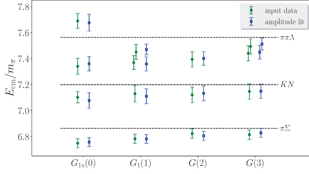
FIG. 3. Finite-volume spectrum in the center-of-mass frame used as input data to constrain parametrizations of the coupled-channel \pi\Sigma - \bar{K}N scattering amplitude. Each column corresponds to a particular irrep \Lambda(\mathbf{d}^2) of the little group of total momentum \mathbf{P}^2 = (2\pi/L)^2 \mathbf{d}^2 . Only irreps where the \ell = 0 partial wave contributes are included. Dashed lines indicate various thresholds, as labeled. Model energies from the resultant scattering-amplitude fit are given by blue squares.
