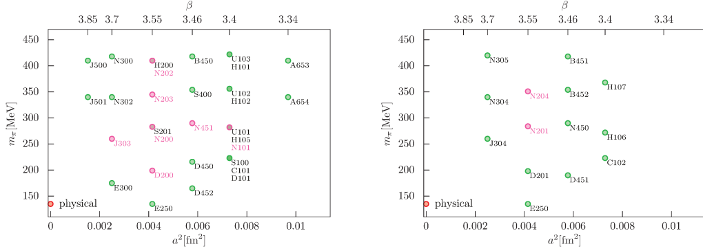
Figure 1: Overview of gauge field ensembles generated by the CLS consortium along quark-mass trajectories with constant trace of the quark-mass matrix (left pane) and along a trajectory where the strange-quark mass has been fixed to its physical value (rhs pane). The ensembles highlighted with magenta color will be used in the current project.
