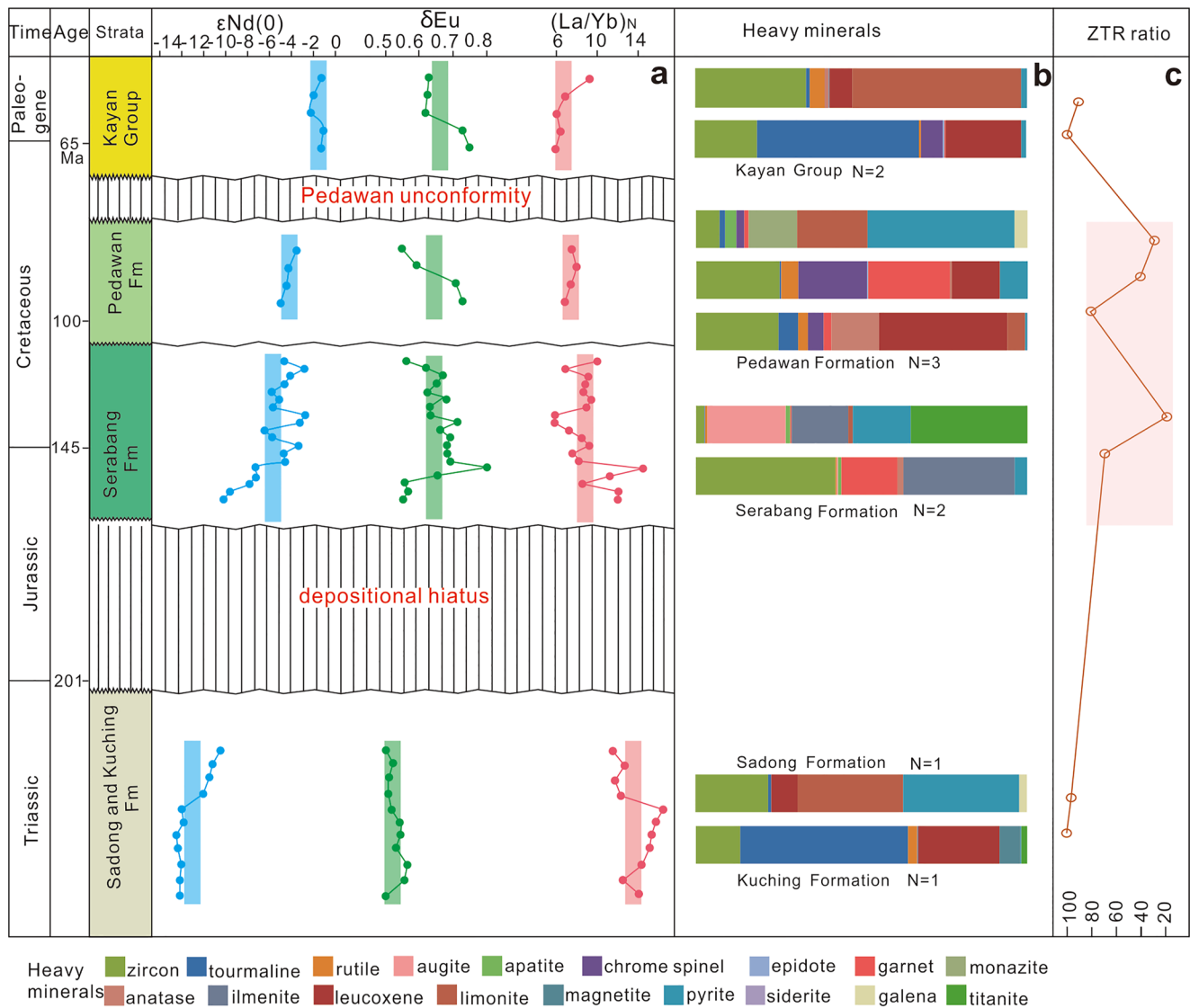
Figure 2. (a) Plot of \epsilon_{Nd}(0) , \delta Eu and (La/Yb)_N values of mudstone samples. Part of the Serabang Formation (Lubok Antu Melange) is from Zhao et al. (2021). (b) Heavy mineral abundance in the sediments. (c) Sample ZTR ratio.
