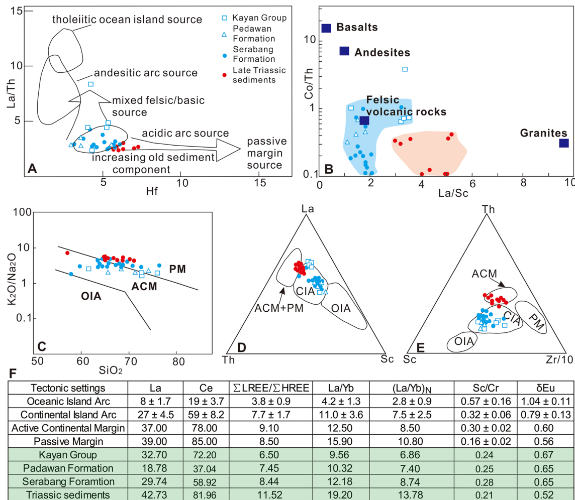
Figure 3. (a) Hf-La/Th plot (Floyd & Leveridge, 1987), (b) La/Sc-Co/Th plot (Gu et al., 2002), (c) K 2 O/Na 2 O-SiO 2 plot (Roser & Korsch, 1986), (d) La-Th-Sc plot, (e) Th-Sc-Zr/10 plot (Bhatia & Crook, 1986). OIA: Oceanic Island Arc; CIA: Continental Island Arc; ACM: Active Continental Margin; PM: Passive Margin. (f) Tectonic background of the sedimentary rocks from West Sarawak (Bhatia, 1985). The La, Ce value of the mudstone was divided by 1.2 to obtain the correction equivalent to that of the graywackes (W. L. Xu et al., 2013; Z. J. Xu et al., 2013). Part of the Serabang Formation (Lubok Antu Melange) is from Zhao et al. (2021).
