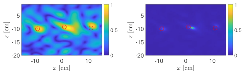
Figure 10. [Left] The image formed through evaluation of the Kirchhoff migration (KM) imaging function (Equation 10) for three targets. The exact target locations are plotted as a red “O” symbol. [Right] The image formed through evaluation of the modified KM imaging function (Equation 15) with \delta = 10^{-2} . Measurement noise is added so that SNR = 24.2 dB.
