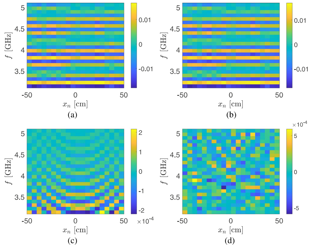
Figure 5. Real part of the entries of (a) the data matrix D , (b) the ground bounce signals R , (c) the scattered signals S , and (d) the matrix \bar{D} with the contributions from the first 5 singular values removed.
