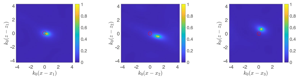
Figure 11. Evaluation of the modified Kirchhoff migration imaging function (Equation 15) with \delta = 10^{-2} in sub-regions centered about each target location.
