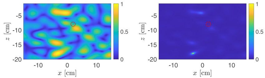
Figure 9. [Left] Kirchhoff migration (KM) image and [Right] modified KM image with \delta = 10^{-2} for a target located at (2, -8) cm with SNR = 14.2 dB and eSNR = -7.0 dB.
