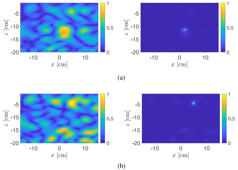
Figure 7. [Left] The image formed through evaluation of the Kirchhoff migration (KM) imaging function (Equation 10). The exact target location is plotted as a red “ \odot ” symbol. [Right] The image formed through evaluation of the modified KM imaging function (Equation 15) with \delta = 10^{-2} . The top row is for a target located at (2, -12) cm and the bottom row is for a target located at (2, -16) cm.
