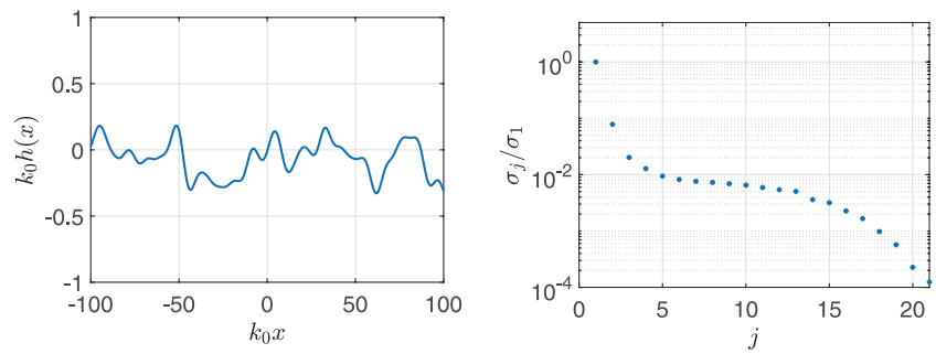
Figure 3. [Left] One realization of the Gaussian-correlated random rough surface with h_{\text{RMS}} = 0.2 cm and \ell = 8 cm with k_0 denoting the wavenumber at the central frequency. [Right] The singular values of the ground bounce signals by this rough surface normalized by the first singular value \sigma_1 .
