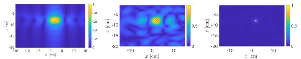
Figure 6. [Left] The ideal image formed through evaluation of the Kirchhoff migration (KM) imaging function (Equation 10) applied to the scattered signals contained in S . [Center] The image formed through evaluation of Equation 10 applied to \bar{D} . [Right] The image formed through evaluation of the modified KM imaging function (Equation 15) with \delta = 10^{-2} applied to the KM image in the center. In each of the plots, the exact target location is plotted as a red “⊙” symbol.
