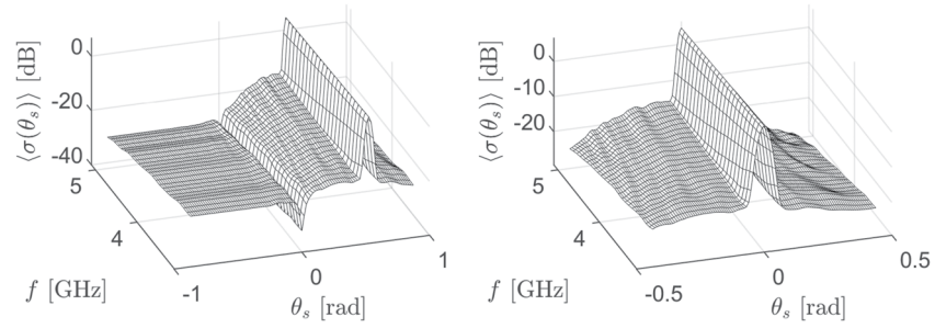
Figure 2. [Left] Average of the bistatic cross-section, \langle \sigma(\theta_s, \theta_i) \rangle , over 100 realizations of a Gaussian-correlated random rough surface with h_{\text{RMS}} = 0.2 cm and \ell = 8 cm due to a plane wave incident with \theta_i = 30^\circ . [Right] A close-up of this result about \theta_s = \theta_i .
