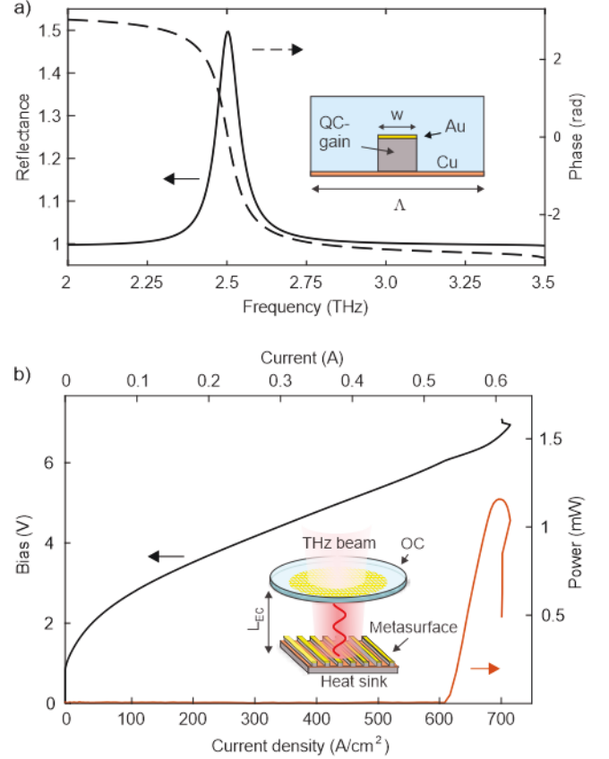
Fig. 1. (a) FEM simulated magnitude and phase of the metasurface reflectance with 20\ \text{cm}^{-1} gain applied to the QC material. Metasurface structure is illustrated in the inset. (b) Measured lasing characteristics of the resulting QC-VECSEL, illustrated in inset.
