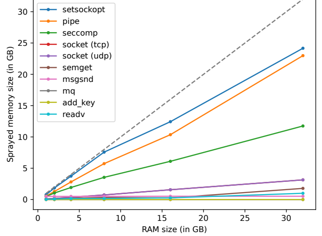
Figure 4: Effectiveness of spraying using different syscalls.
